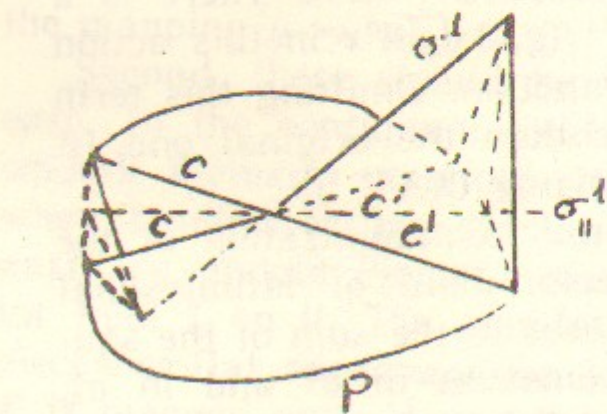
Fig. 1. The two alternative cuts c and c' relevant to the two different maximal continuous plane-like extensions of the surface P around the curvature support \sigma^1 (in the three dimensional space); \sigma_{\parallel}^1 is the projection of \sigma^1 onto P .
