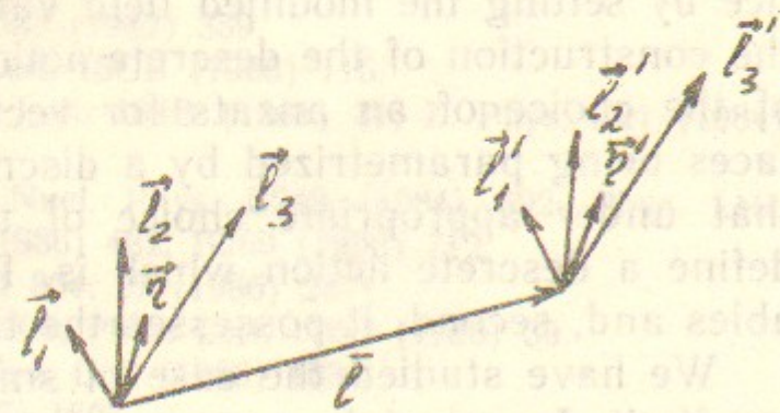
Fig. 3. Vectors \tilde{\eta} , \tilde{\eta}' on periodic Regge lattice; \bar{l}_a , \bar{l}'_a , \bar{l} are the edges.
