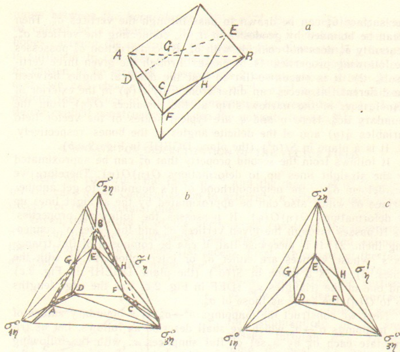
Fig. 2. Construction of the face \sigma_n^2 . a). DGEHF is a plane close to the face \sigma^2 = ABC inside the union St(\sigma^2) of the two tetrahedra having ABC as the common face. D, G, E, H, F are intersections of this plane with the edges \sigma^1 \subset St(\sigma^2) carrying the curvature (another edges not belonging St(\sigma^2) are not shown for simplicity). b). The piecewise-flat surface \tilde{\sigma}_n^2 is a maximal continuous extension of DGEHF into the exterior of St(\sigma^2) as a plane. Solid lines divide \tilde{\sigma}_n^2 into a set of the flat simplices; of these lines the double ones are the cuts symmetric with respect to the projections of curvature supports \sigma_n^1 shown by dotted lines (see Fig. 1). c). The piecewise-flat surface \tilde{\sigma}_n^2 bounded by straight lines is obtained by deformation of \tilde{\sigma}_n^2 near it's boundary (in the exterior of St(\sigma^2) ). Solid lines divide \tilde{\sigma}_n^2 into a set of the flat simplices s^2 .
