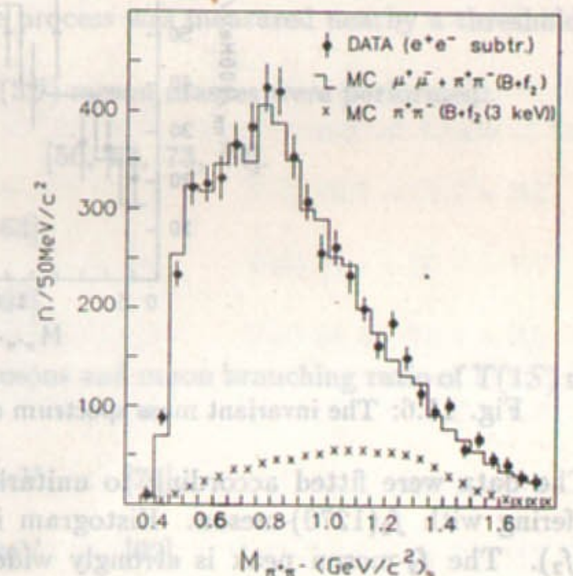
Fig. 11.5: The invariant mass spectrum of pairs after rejection of electrons.
