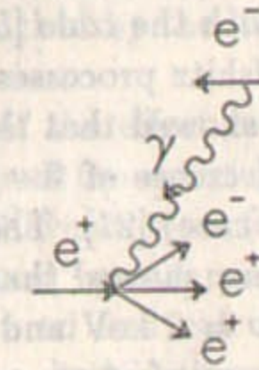
Fig. 3.4: Schematic view of the process \gamma e \rightarrow ee^+e^- .
