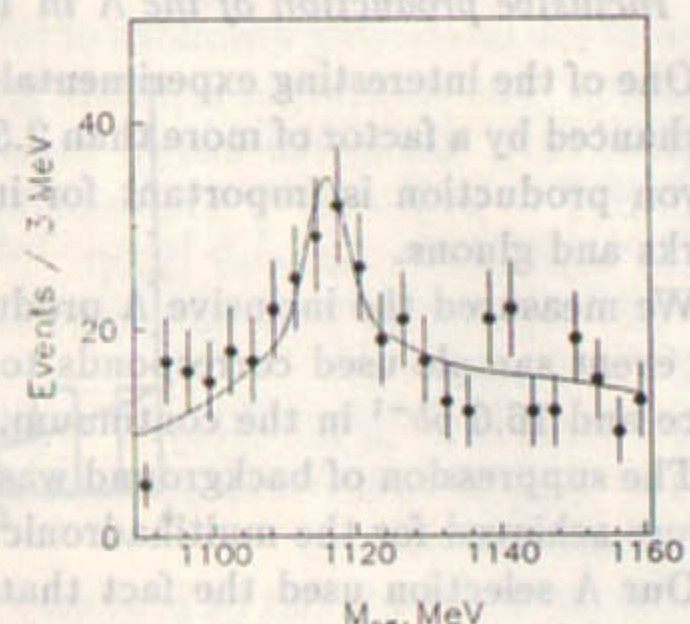
Fig. 7.2: p\pi^- invariant mass distribution for the continuum.
