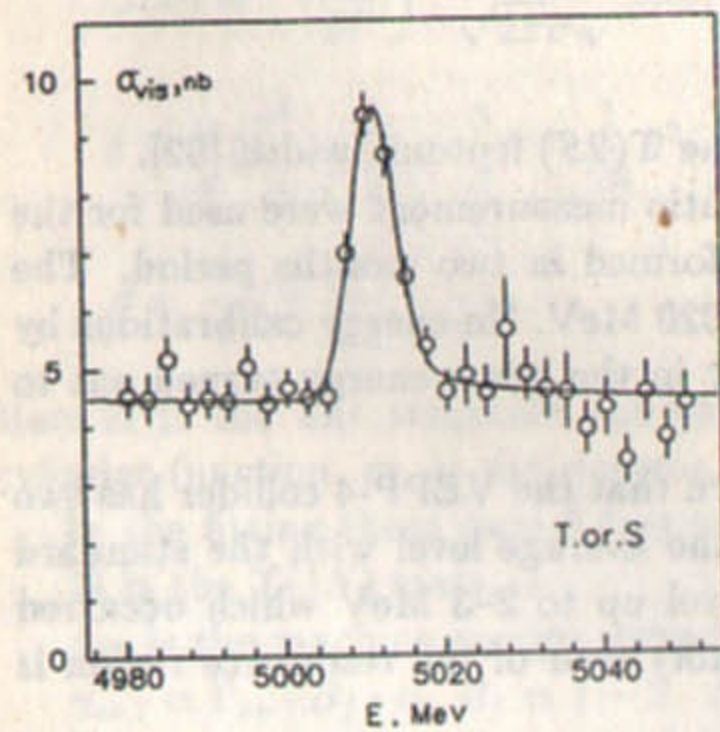
Fig. 5.3: The visible cross section for e^+e^- \rightarrow hadrons with T.or.S selection criterion in the \Upsilon(2S) region.
