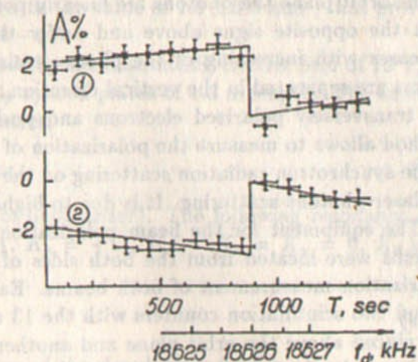
Fig. 4.2: Result of one of the depolarization frequency measurements. 1 and 2 - SR scattering on e^- and e^+ beams. A = (\text{up-down})/(\text{up+down}) was averaged over 100 sec. Lower scale shows the depolarizer frequency f_d . Beam currents are I_- = 5.8 mA, I_+ = 6.2 mA.
