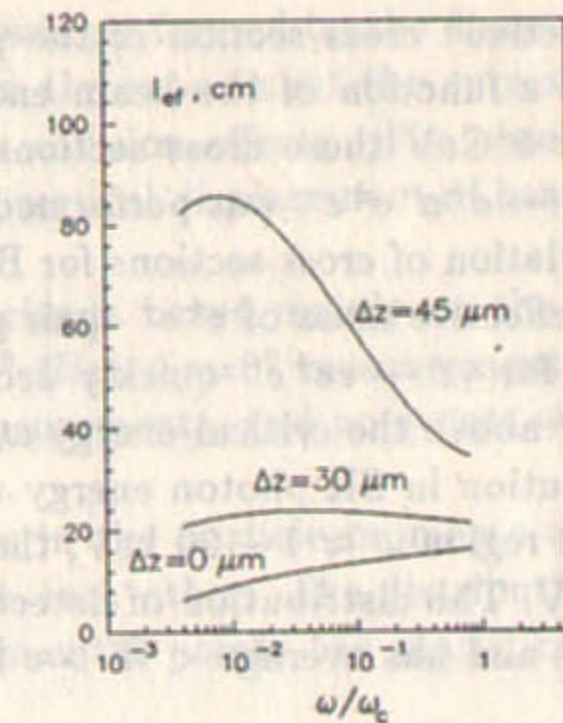
Fig. 3.5: Energy dependence of the effective length l_{ef} for E=5.14 GeV, magnetic field H=12.5 kG, \sigma_z=12.5 \mu\text{m} , \sigma_r=0.07 cm.
