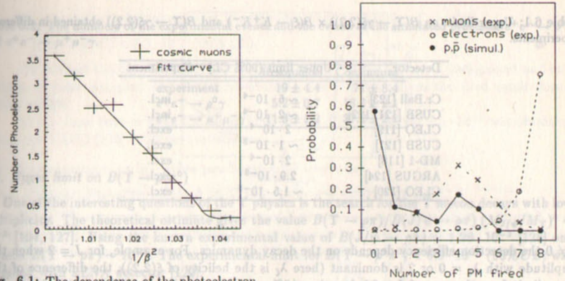
Fig. 6.1: The dependence of the photoelectron number in Cherenkov counters versus the inverse square of the cosmic muons velocity and the fitted curve
