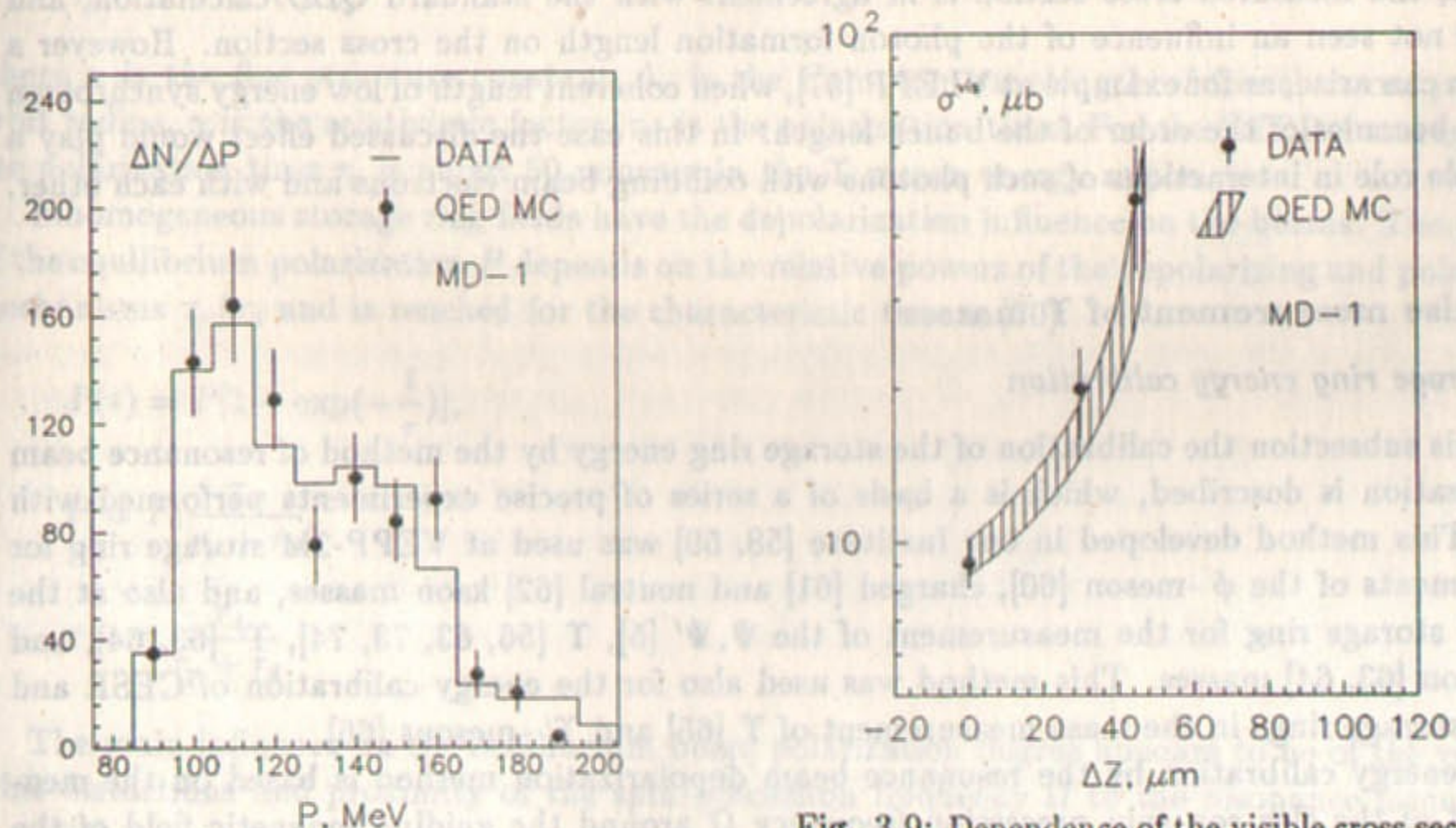
Fig. 3.9: Dependence of the visible cross section \gamma e \rightarrow ee^+e^- + e^+e^- \rightarrow e^+e^-e^+e^- on the vertical displacement of beams for one experimental run. \sigma_z = 13 \pm 0.5 \mu\text{m} .
