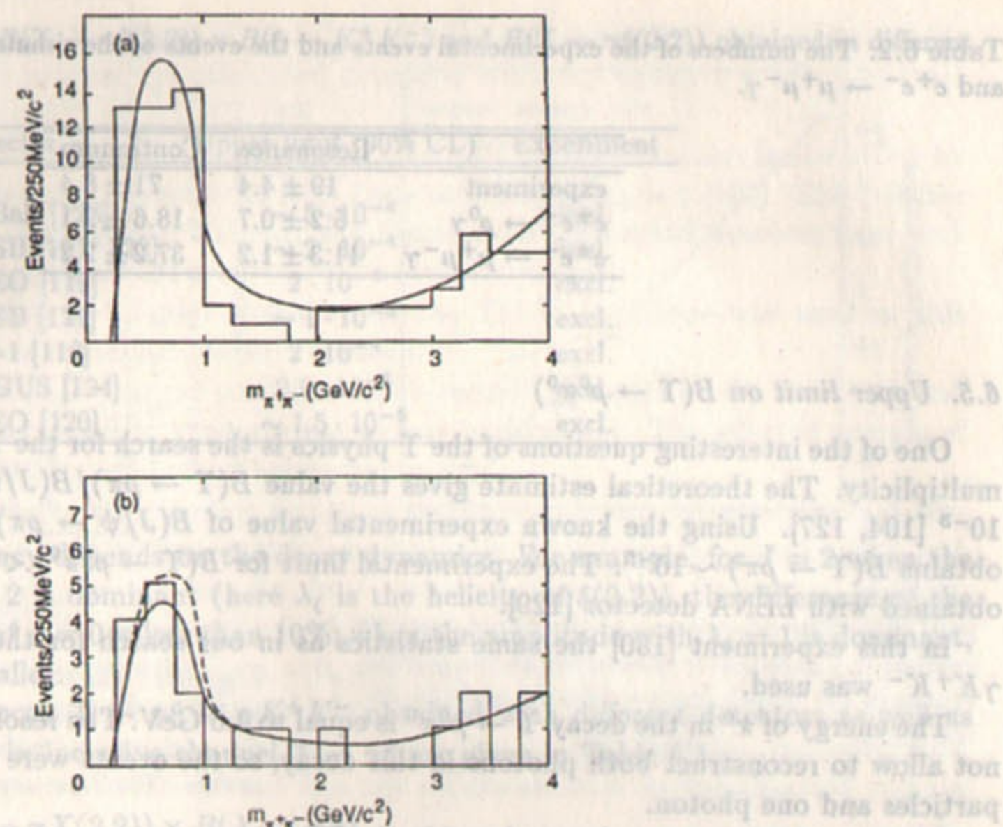
Fig. 6.3: Distribution of experimental events in m_{\pi^+\pi^-} and fitted curves. (a) Events outside the resonance region are shown. (b) Events in the resonance region are shown. The dashed line displays the fitted curve including the decay \Upsilon \rightarrow \rho^0 \pi^0 with probability B(\Upsilon \rightarrow \rho^0 \pi^0) = 3.3 \cdot 10^{-4} in addition to the background processes.
