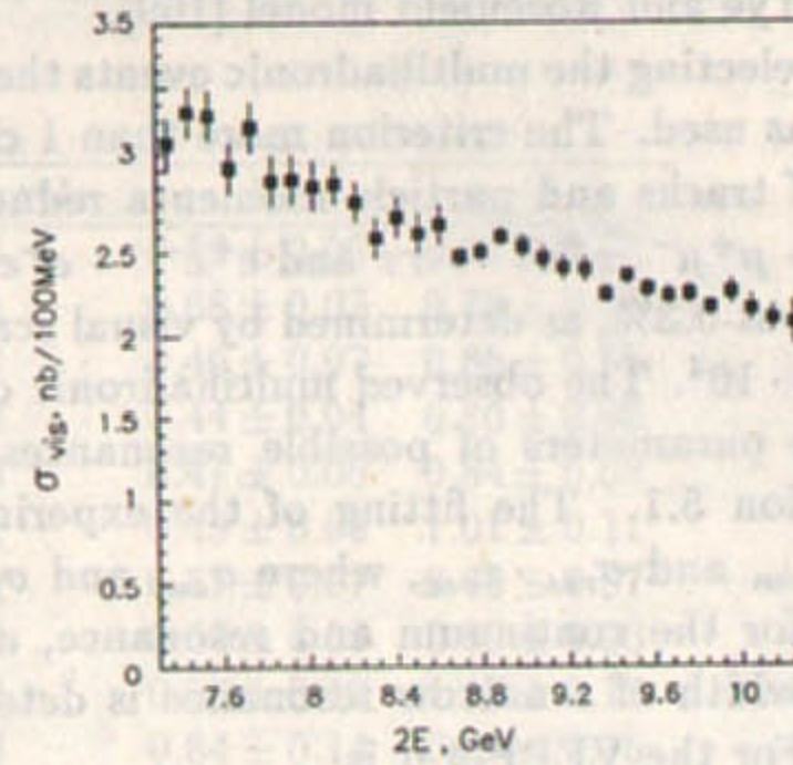
Fig. 9.2: The visible cross section of e^+e^- \rightarrow \text{hadrons} versus center-of-mass energy.
