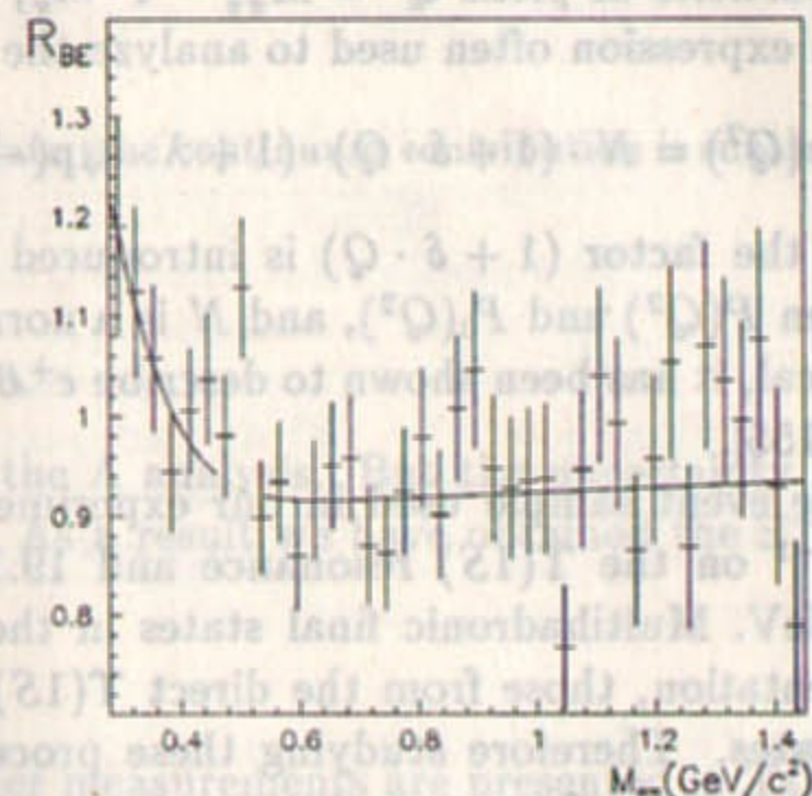
Fig. 8.2: Continuum: r_{data}/r_{MC} , corrected.
