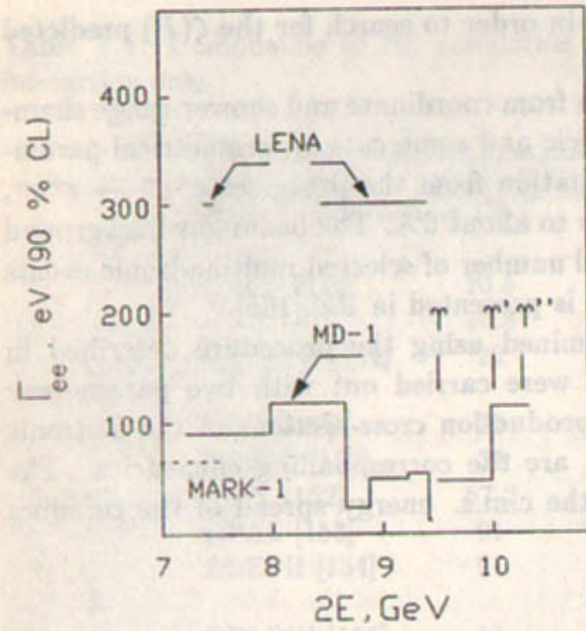
Fig. 9.1: Upper limits on \Gamma_{ee} for narrow resonances (90% CL). Data from MARK-1 [165] (dashed line), LENA [79], and MD-1 [165]
