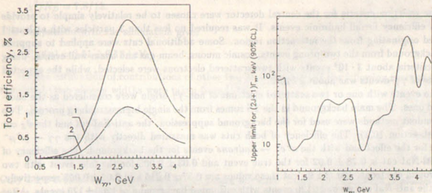
Fig. 10.12: The total selection efficiency in the double-tag mode for narrow resonances vs resonance invariant mass. 1- anti-NaI cut, 2- anti-NaI cut and \vartheta_Z cut.
