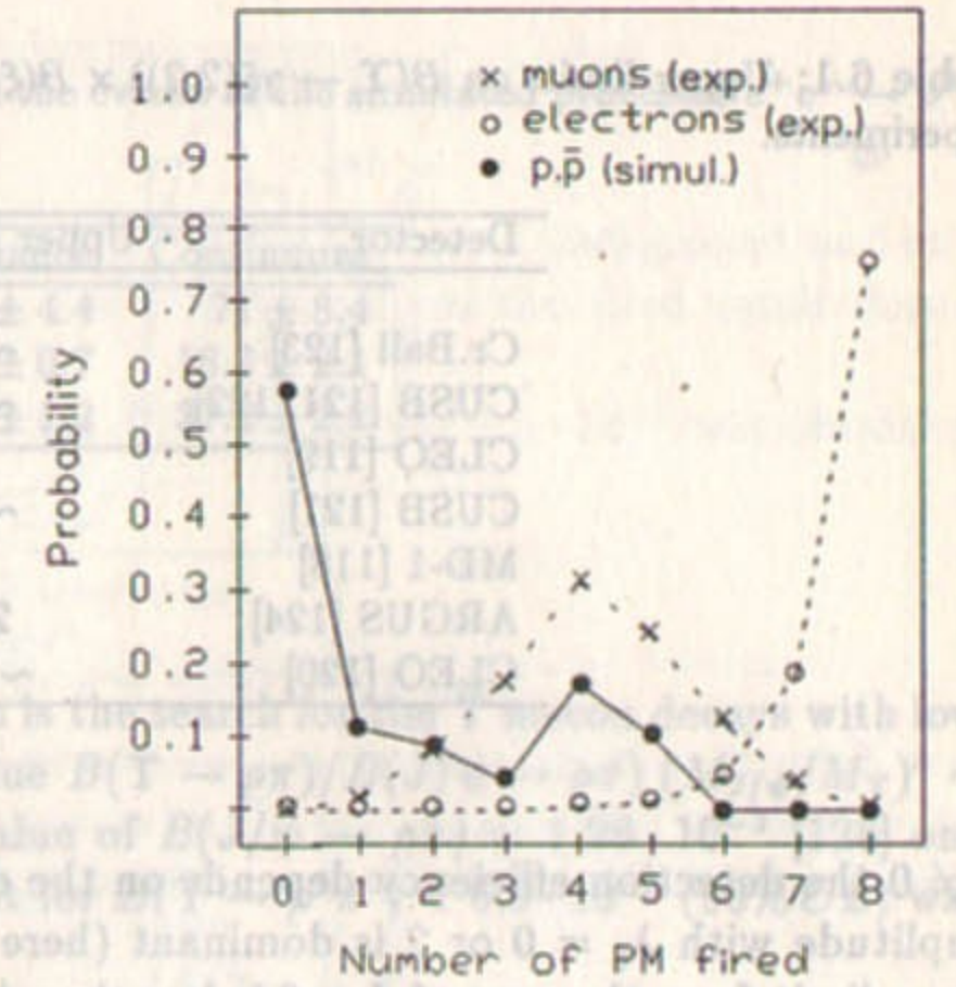
Fig. 6.2: The distributions of probability versus the fired PM number in Cherenkov counters for Bhabha events, muon pairs, and simulated p\bar{p} events. The lines are drawn to guide eye.
