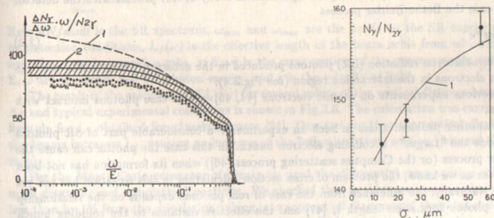
Fig. 3.2: A spectrum of SB photons: dark circles - the experiment in 1980, \sigma_z = 23 \pm 3 \mu m ; open triangles - the experiment in 1981, \sigma_z = 24 \pm 3 \mu m ; 1 - the standard QED calculation; 2 - the calculation taking into account the effect of the large impact parameter cut-off [34, 35].
