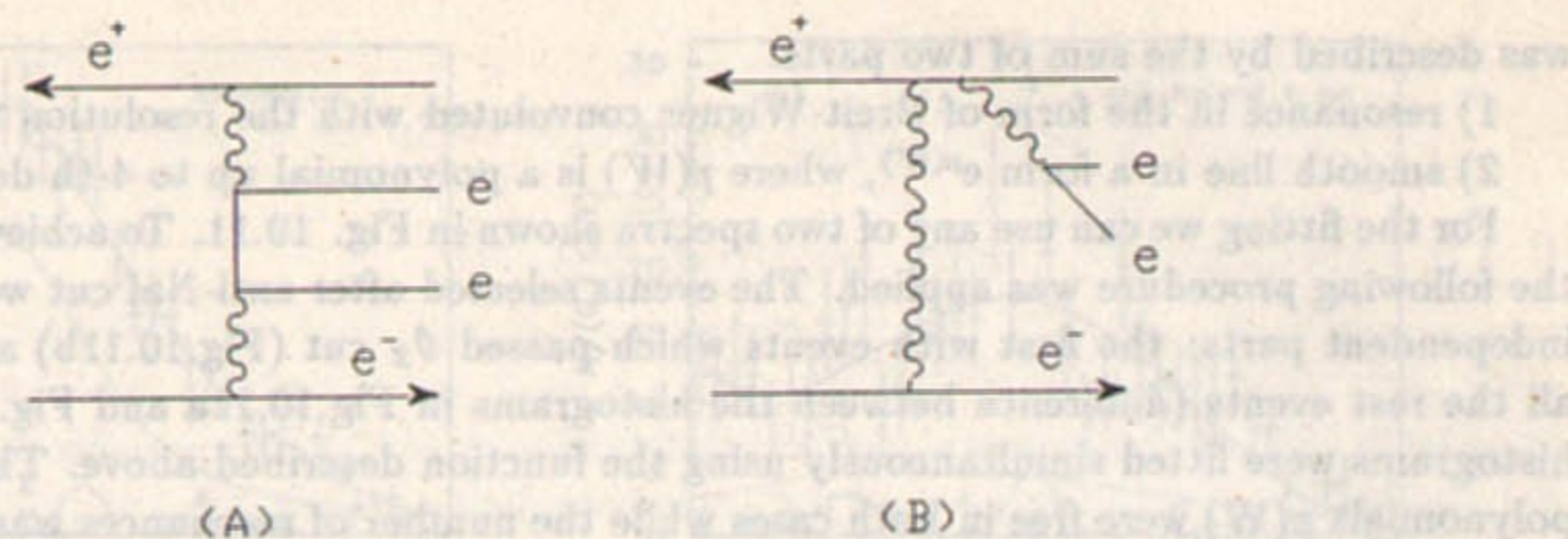
Fig. 11.1: Diagrams for the reaction e^+e^- \rightarrow e^+e^- + e^+e^- : A - the multiperipheral two photon graph; B - the bremsstrahlung graph.
