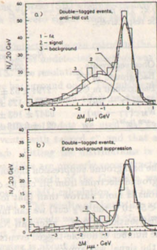
Fig. 10.4: Double-tagged events. Distributions in \Delta M_{\mu\mu} = M_{\mu\mu}^{CD} - M_{\mu\mu}^{TS} . a) Events with anti-NaI cut. Effect/background equals 1.1. b) Events with anti-NaI and \vartheta_z < 0.5 mrad cuts. Effect/background ratio equals 2.3.
