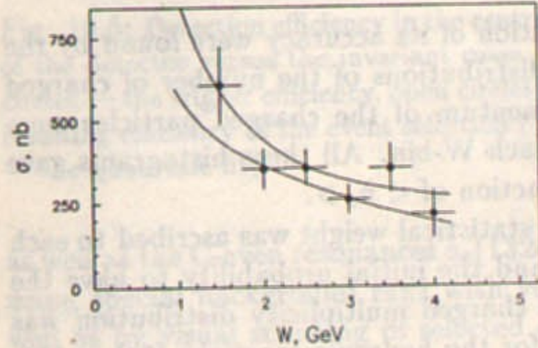
Fig. 10.7: Total cross section of the reaction \gamma\gamma \rightarrow \text{hadrons} versus the invariant mass. Points — experimental data, vertical bars — statistical and systematic errors added in quadrature, horizontal — intervals of the cross section averaging. Lines — A+B/W — fit \pm 1\sigma .
