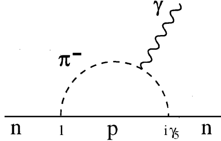
Figure 3: Chiral contribution to the neutron EDM. \pi NN vertices \mathbf{1} and i\gamma_5 refer to the CP -odd and usual strong interactions, respectively.
