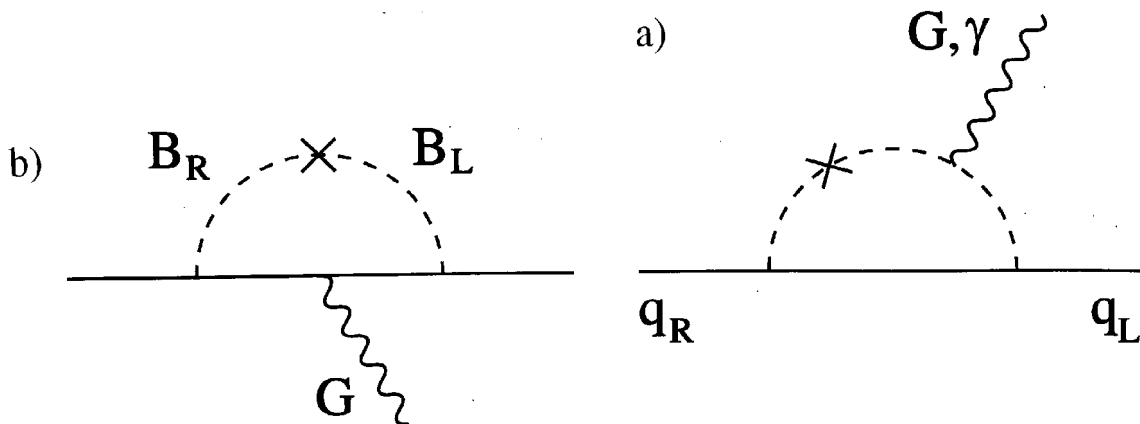
Figure 1: Gluino contributions to quark dipole moments. B_{L(R)} denotes the left(right)-handed b -squark.
