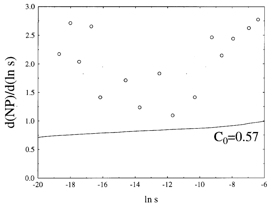
Figure 2: Derivative of the distribution function in Fig.1. Solid line shows dependence (3.6) with the same fitting parameter C_0 = 0.57 .
