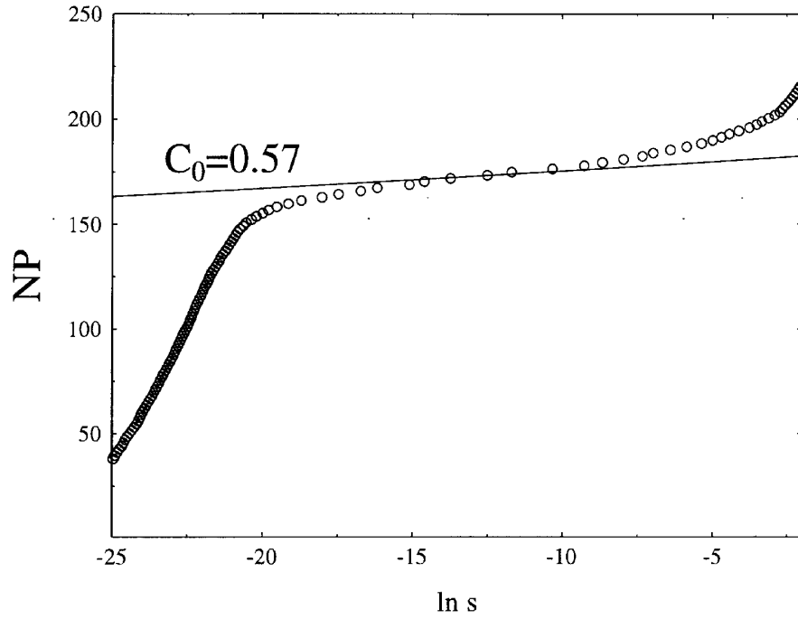
Figure 1: Statistics of quasidegeneracies in model (3.1): k = 6 - 10 ; K \approx 0.15 - 0.25 ; N = 501 (after Ref.[7]). Solid line is the best fit of numerical data[7] to theoretical dependence (3.5) with C = 1/C_0^2 .
