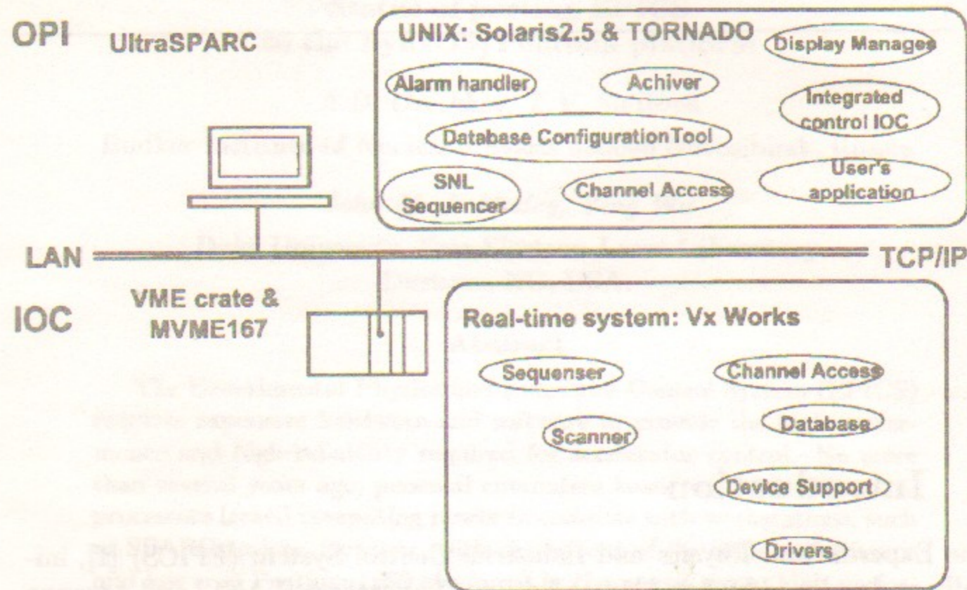
Figure 1: Structure of EPICS.
