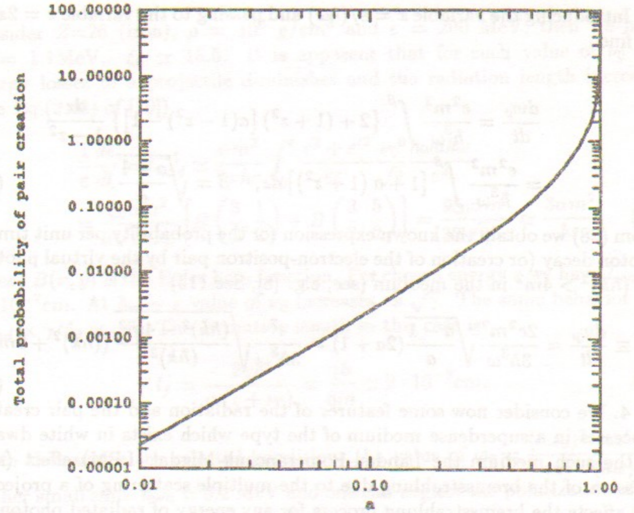
Figure 3: The total probability of the transition pair creation w_p Eq.(23) in units \frac{e^2}{2\pi\hbar} as the function of a = \frac{(\hbar\omega_0)^2}{4m^2} = \frac{(\hbar k)^2}{4m^2} .
