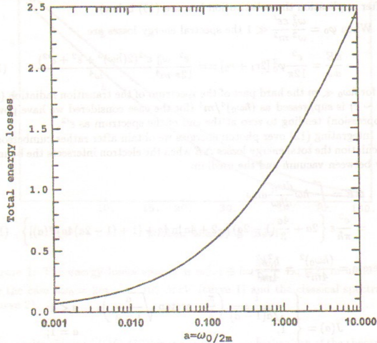
Figure 2: The total energy losses \Delta E Eq.(14) in units \frac{e^2 \varepsilon}{\pi \hbar} when the electron intersects the boundary between vacuum and a medium versus a = \frac{(\hbar \omega_0)^2}{4m^2} = \frac{(\hbar k)^2}{4m^2} .
