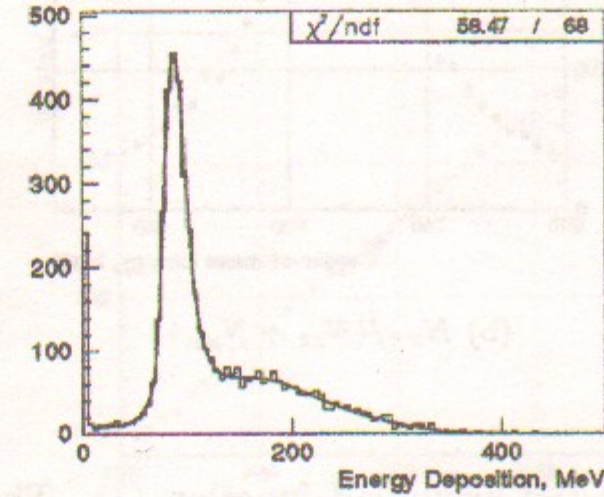
(a) \pi^+ , 345 < E_\pi < 355 \text{ MeV}
