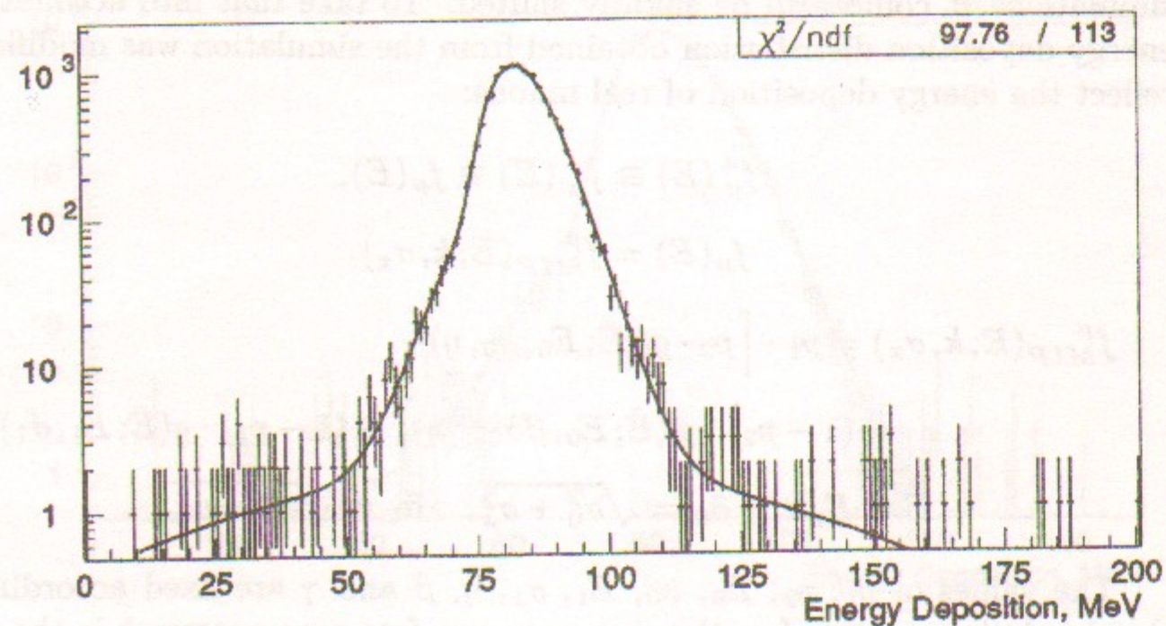
(a) Energy deposition of 400 MeV pions
