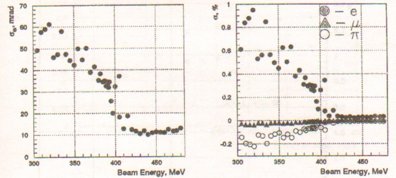
(a) \Theta -resolution
