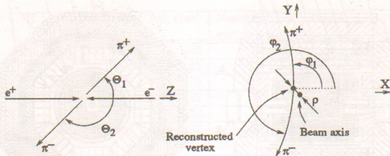
Figure 2: Definition of parameters for two track events
