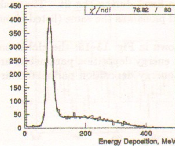
(c) \pi^+ , 425 < E_\pi < 435 \text{ MeV}
