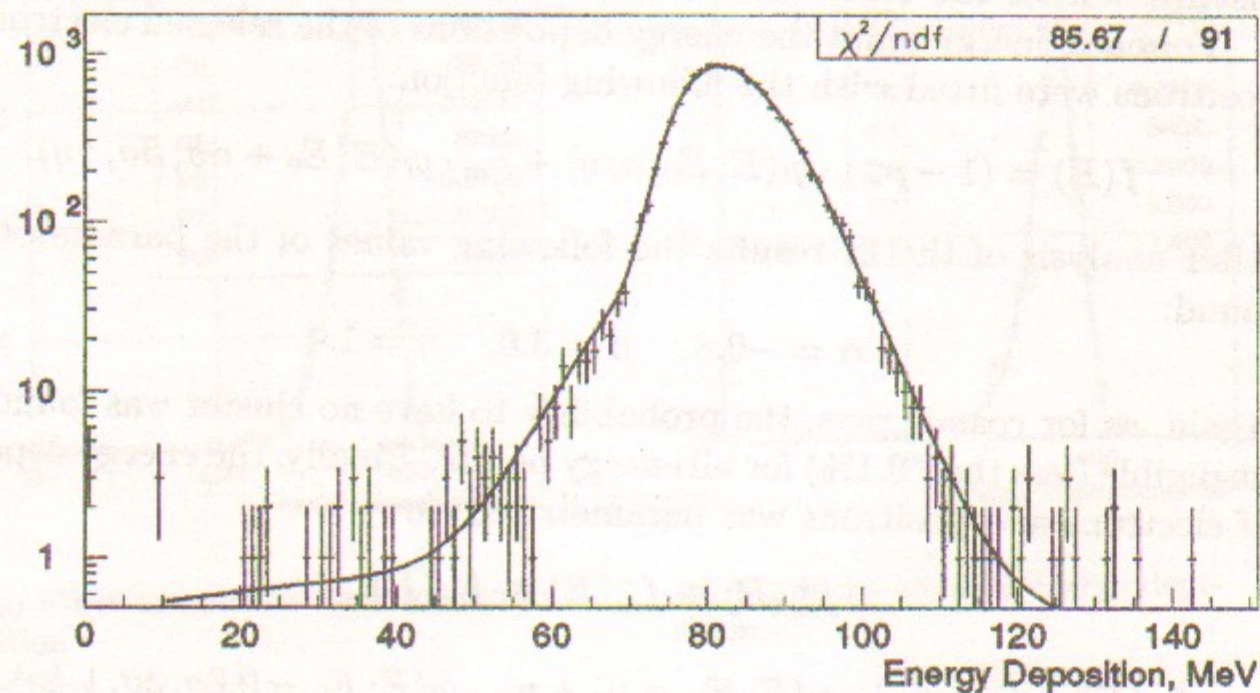
(a) Energy deposition of 375 MeV muons
