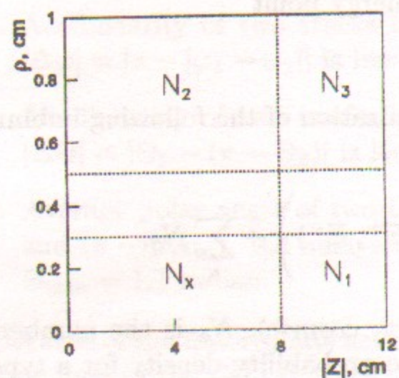
Figure 4: To determination of number of cosmic background events
