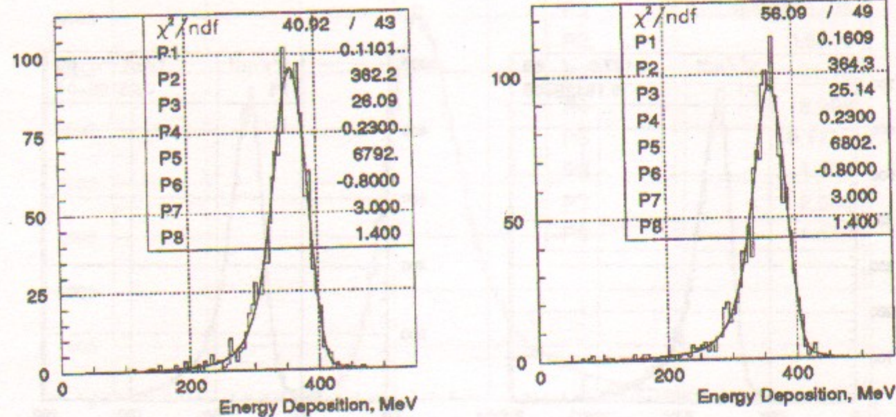
(b) Fit of the electron energy deposition
