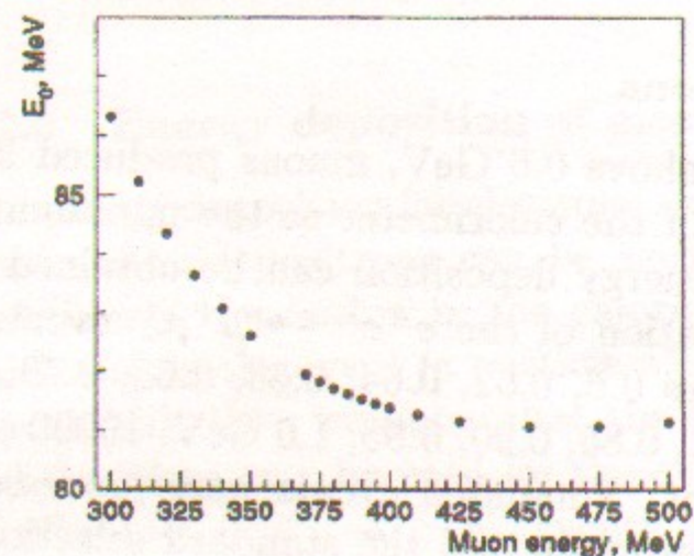
(b) Energy dependence of E_0
