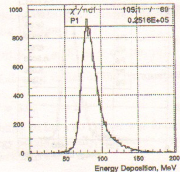
(b) Group 0.71–0.778 GeV
