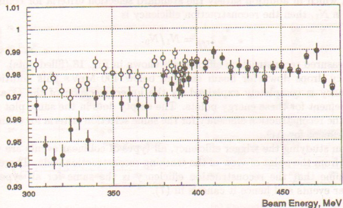
Figure 18: Reconstruction efficiency for all energy points
