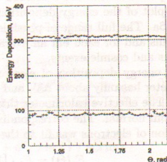
(d) Average energy deposition versus \Theta for electrons and cosmic background events after correction
