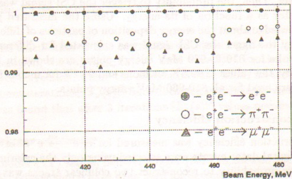
(b) CSI signal efficiency for collinear events
