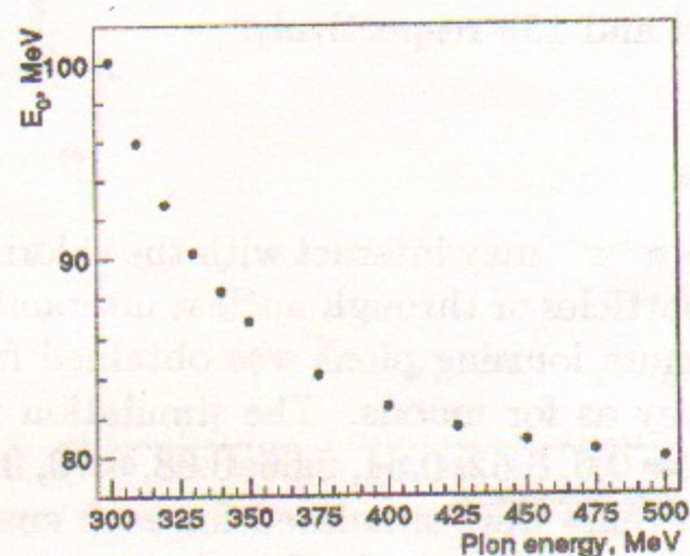
(b) Energy dependence of E_0
