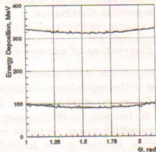
(b) Average energy deposition versus \Theta for electrons and cosmic background events before correction
