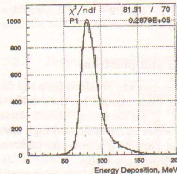
(c) Group 0.780–0.810 GeV
