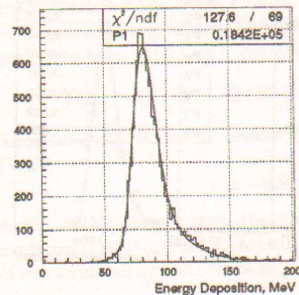
(a) Group 0.61–0.70 GeV
