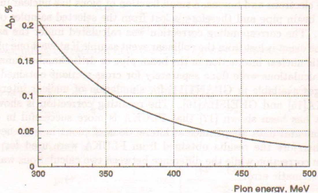
Figure 21: The probability \Delta_D to lose the e^+e^- \rightarrow \pi^+\pi^- event from the sample of collinear events due to pion decay in flight
