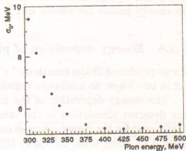
(c) Energy dependence of \sigma_0
