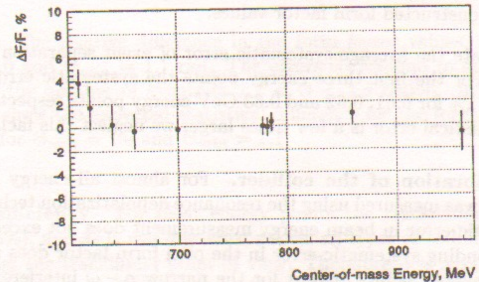
(b) The relative difference between simulated and reconstructed form factor values for the complete detector simulation of collinear events
