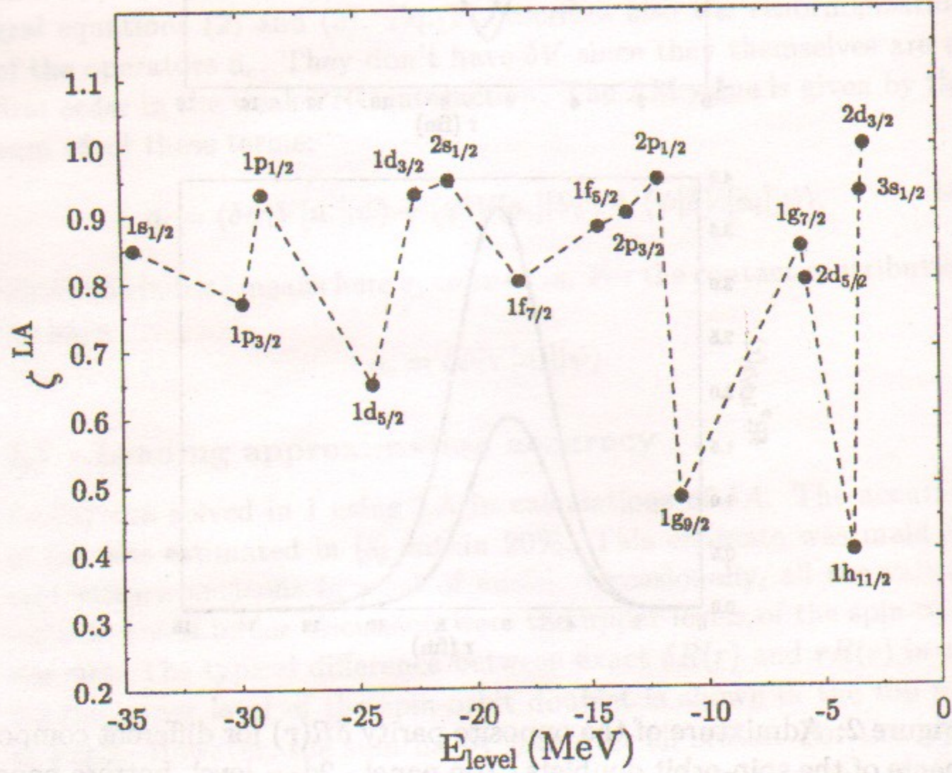
Figure 3: Ratio \zeta of the maximum in exact \delta R(r) to the maximum in rR(r) found in LA for a set of the proton single-particle orbitals.
