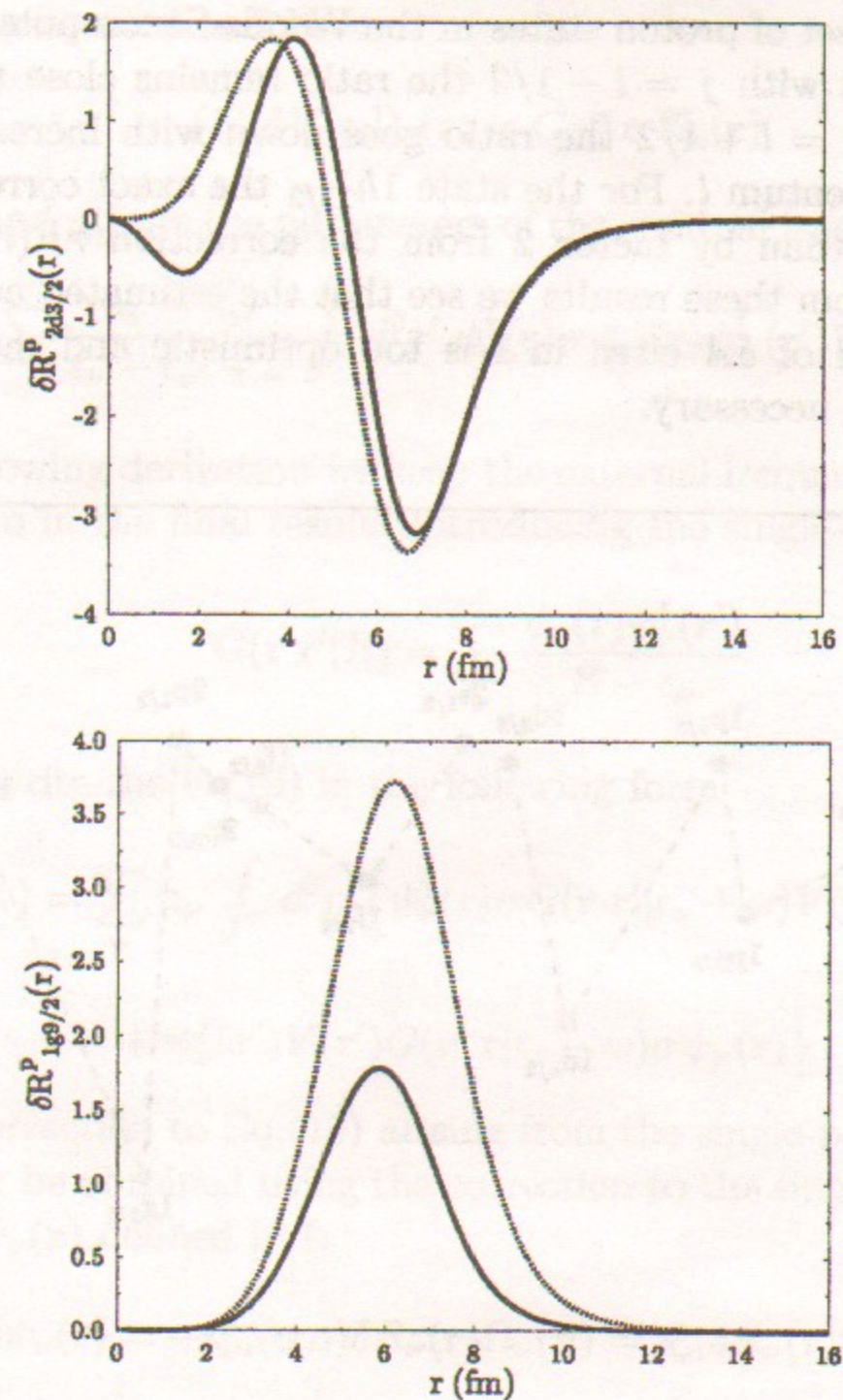
Figure 2: Admixture of the opposite parity \delta R(r) for different components of the spin-orbit doublets. Top panel - 2d_{3/2} level, bottom panel - 1g_{9/2} level. LA is shown by the dashed lines. Full lines show the exact solution.
