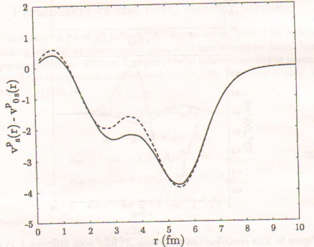
Figure 4: The difference v_s^p(r) - v_{0s}^p(r) for the spin part of the AM operator in the presence of pairing (solid line), and in the absence of pairing (dashed line).
