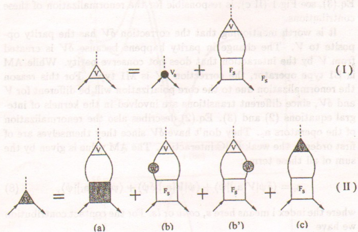
Figure 1: Feynman diagrams corresponding to Eqs.(2),(3).
