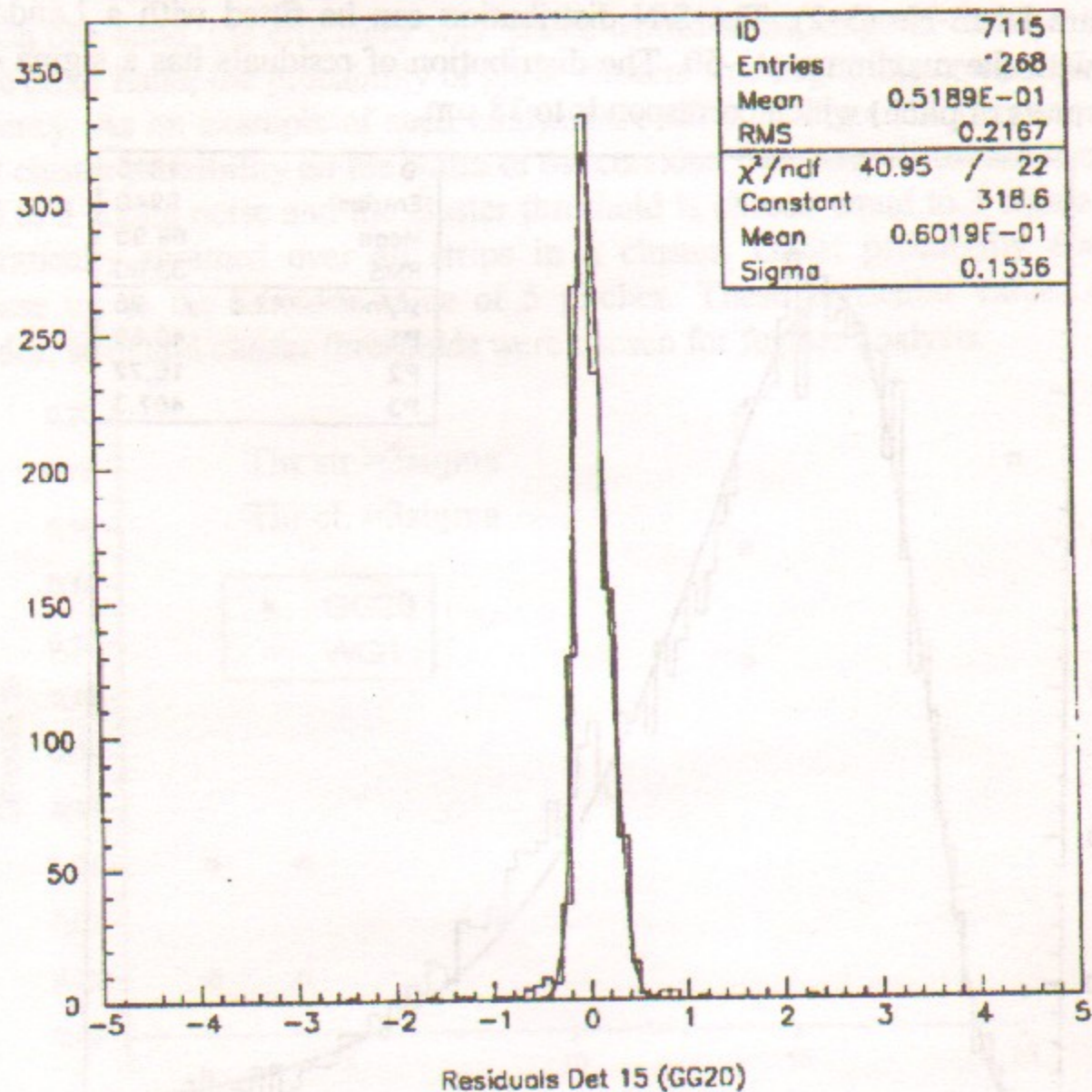
Fig. 6. Distribution of the residuals for GG20.
