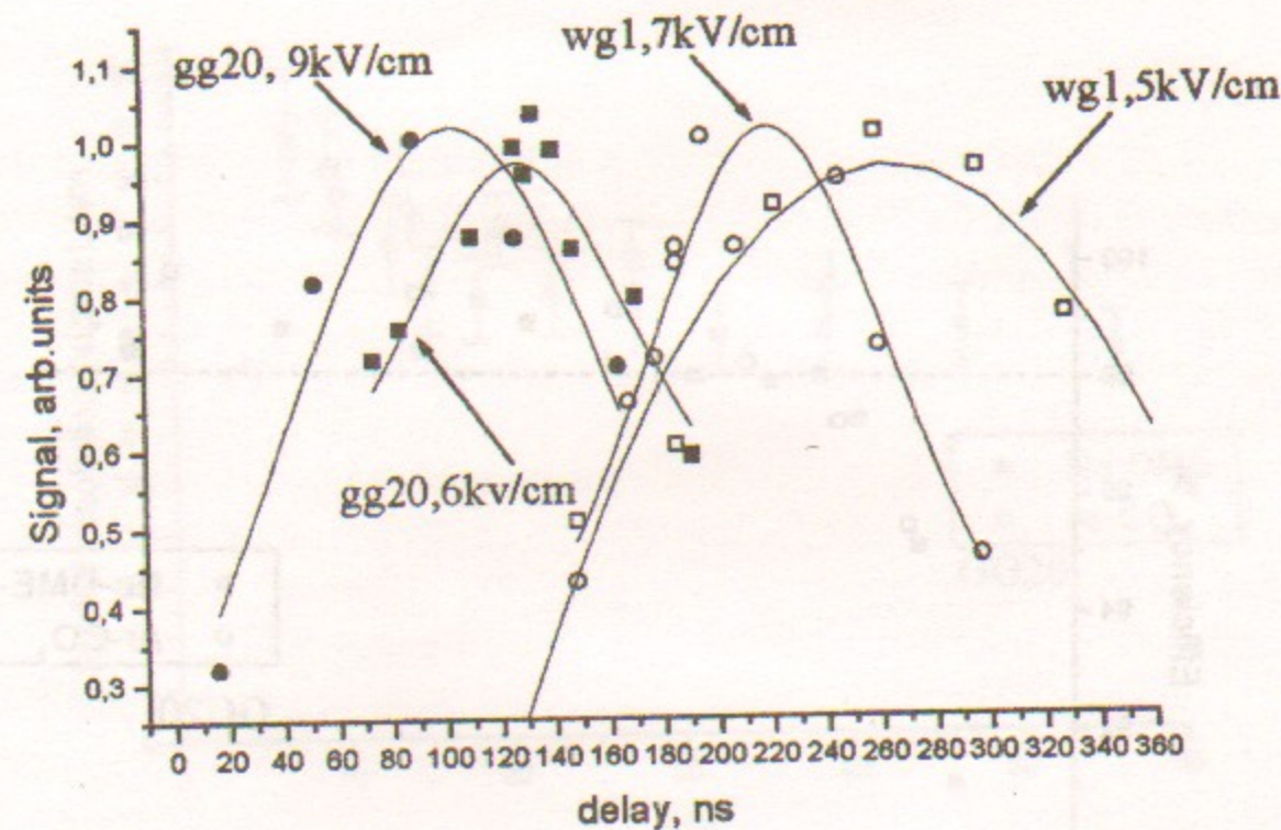
Fig. 7. Delay curves for Ne-DME.
