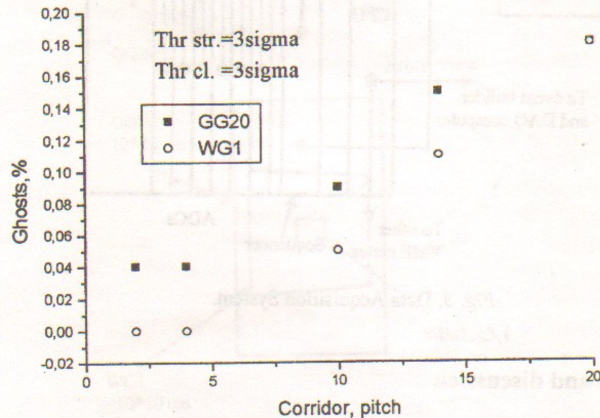
Fig. 4. Justification of the selection algorithm.
