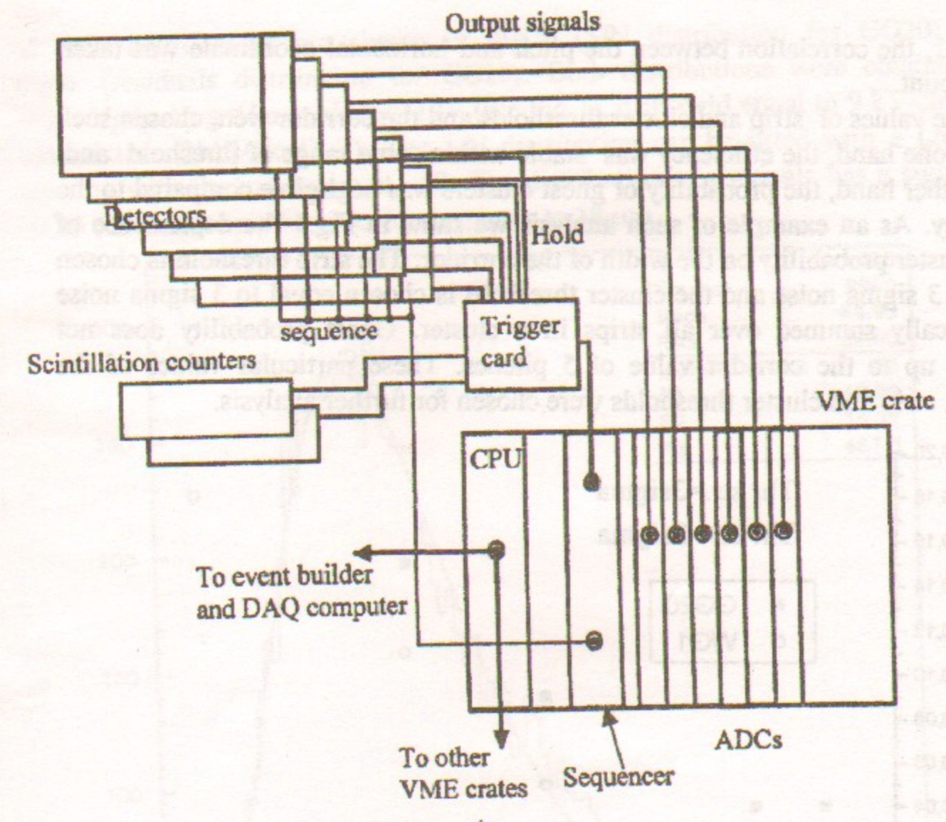
Fig. 3. Data Acquisition System.
