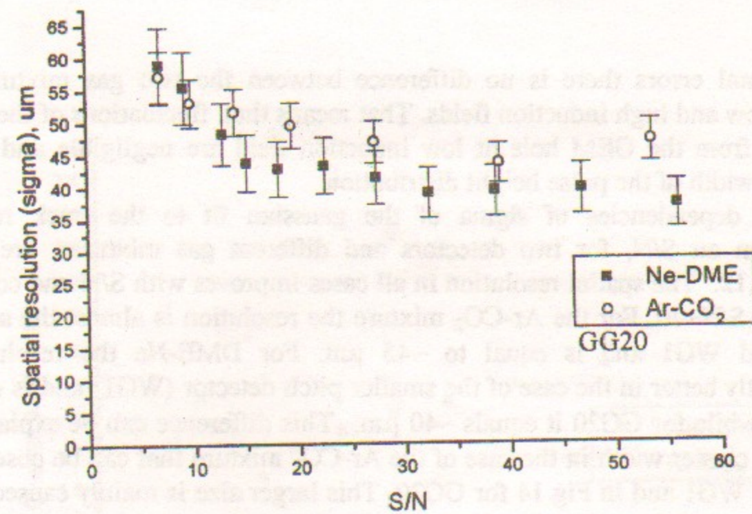
Fig. 11. Spatial resolution vs S/N for GG20.
