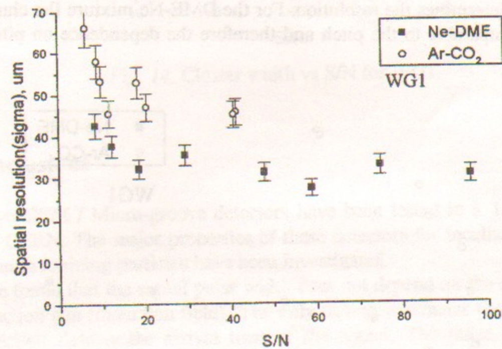
Fig. 12. Spatial resolution vs S/N for WG1.
