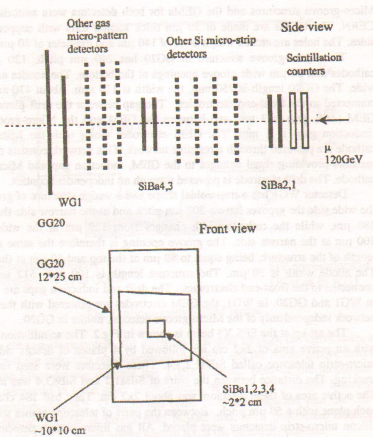
Fig. 2. Set-up at X5.
