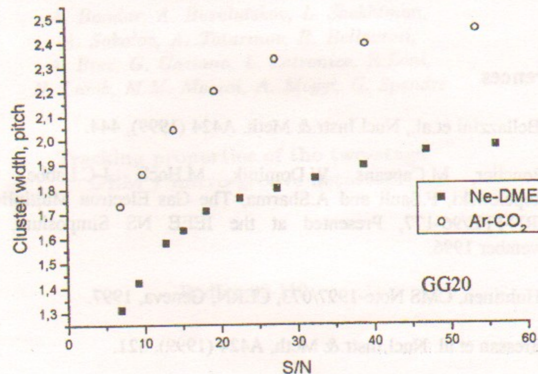
Fig. 14. Cluster width vs S/N for WG1.
