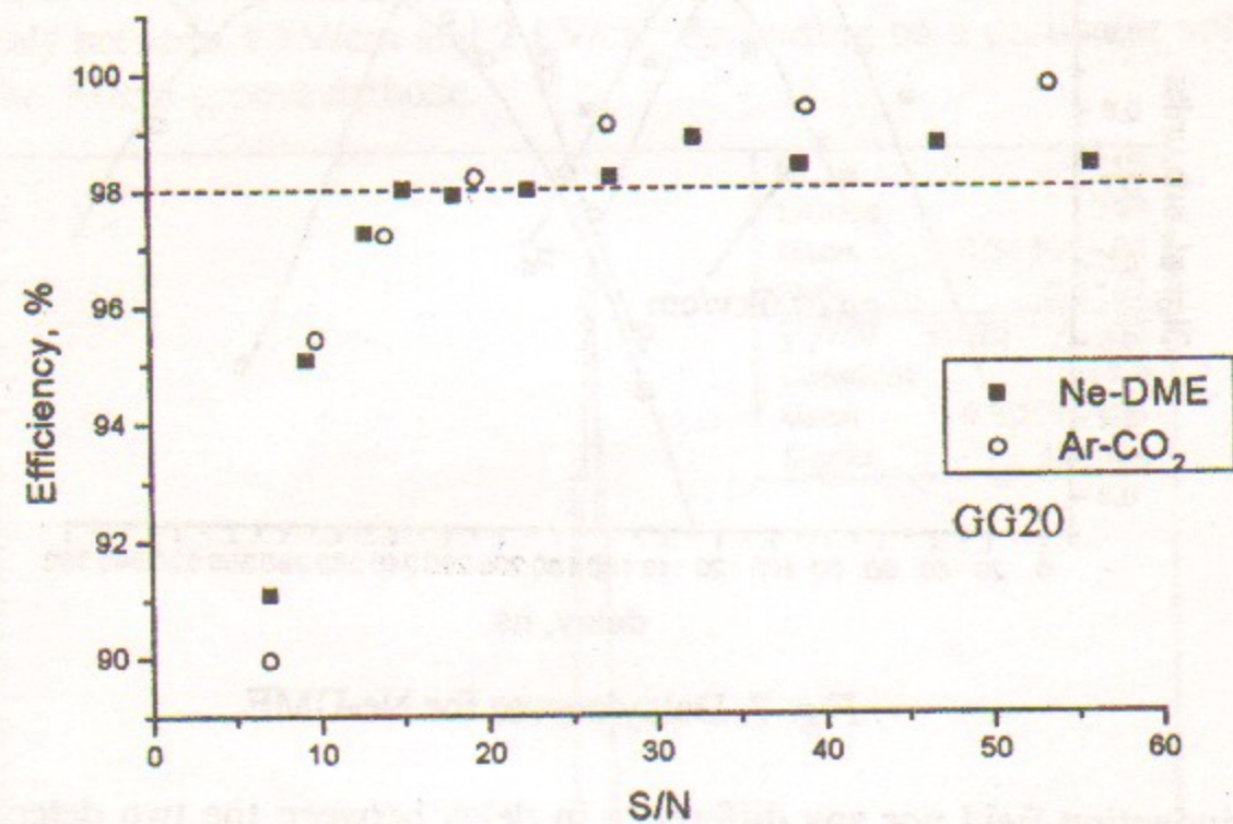
Fig. 9. Efficiency vs S/N for GG20.
