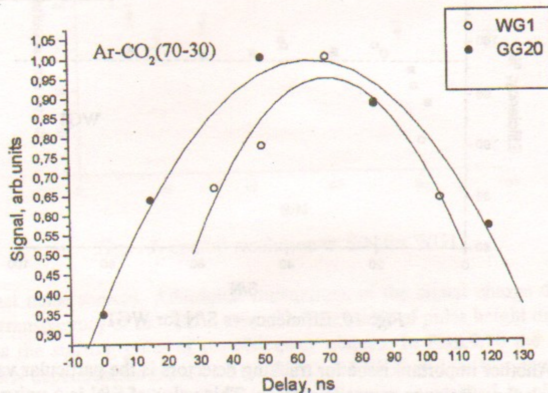
Fig. 8. Delay curves for Ar-CO 2 .
