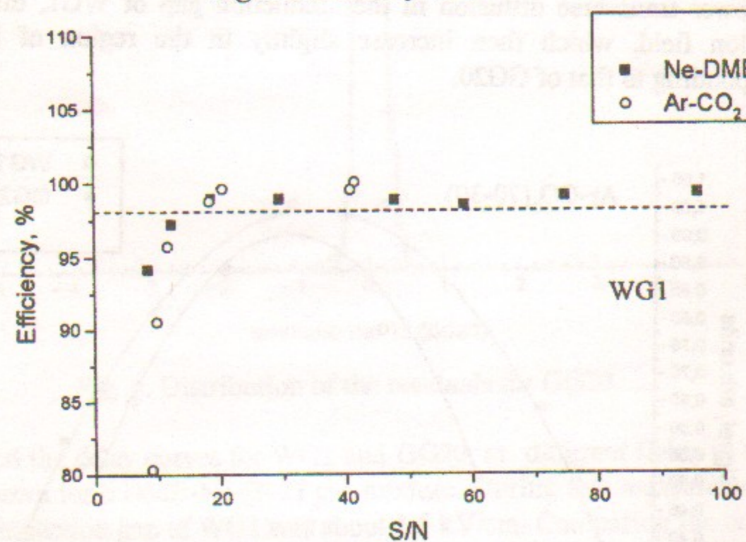
Fig. 10. Efficiency vs S/N for WG1.
