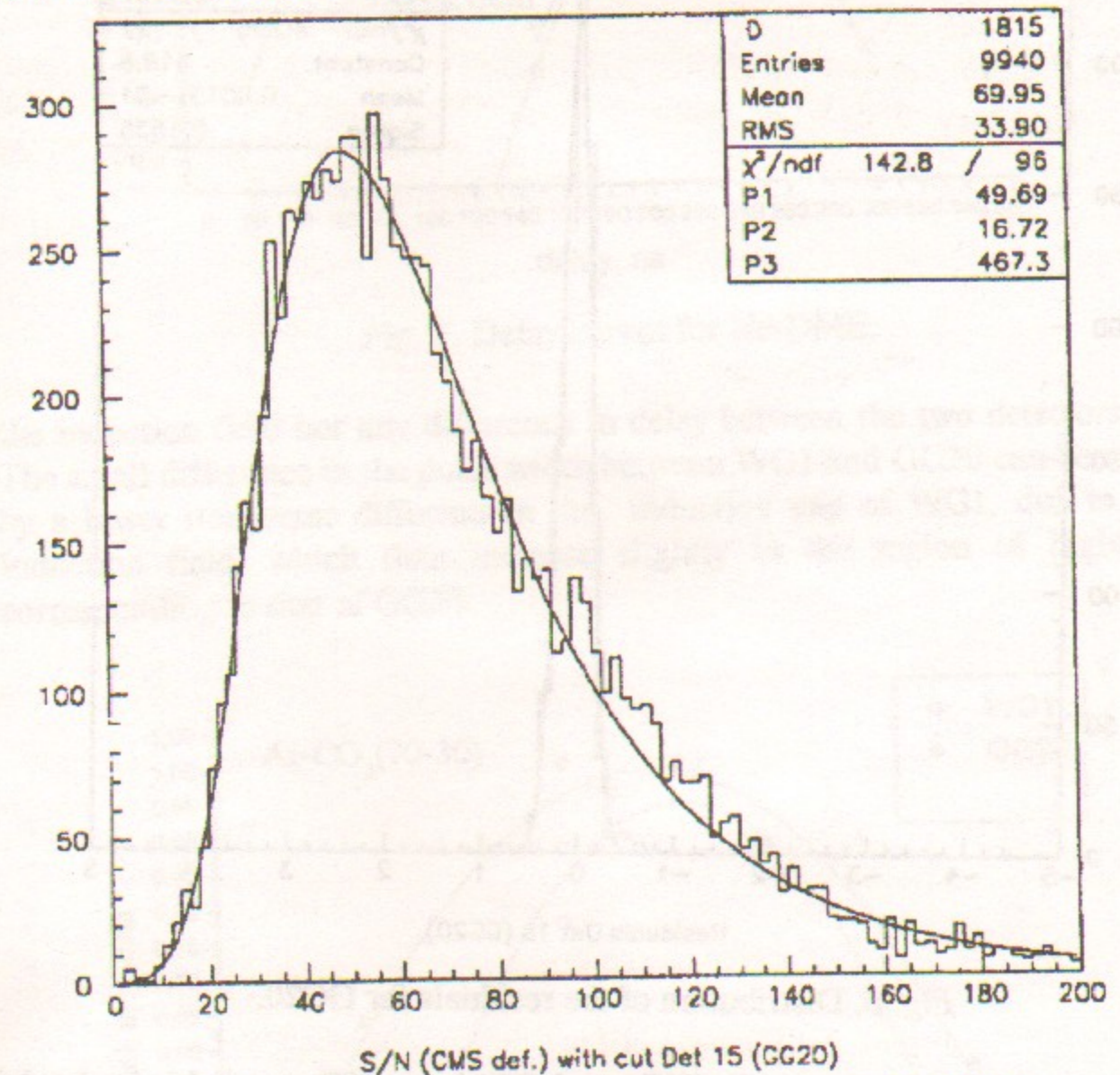
Fig. 5. Distribution of the signal over noise values for GG20.
