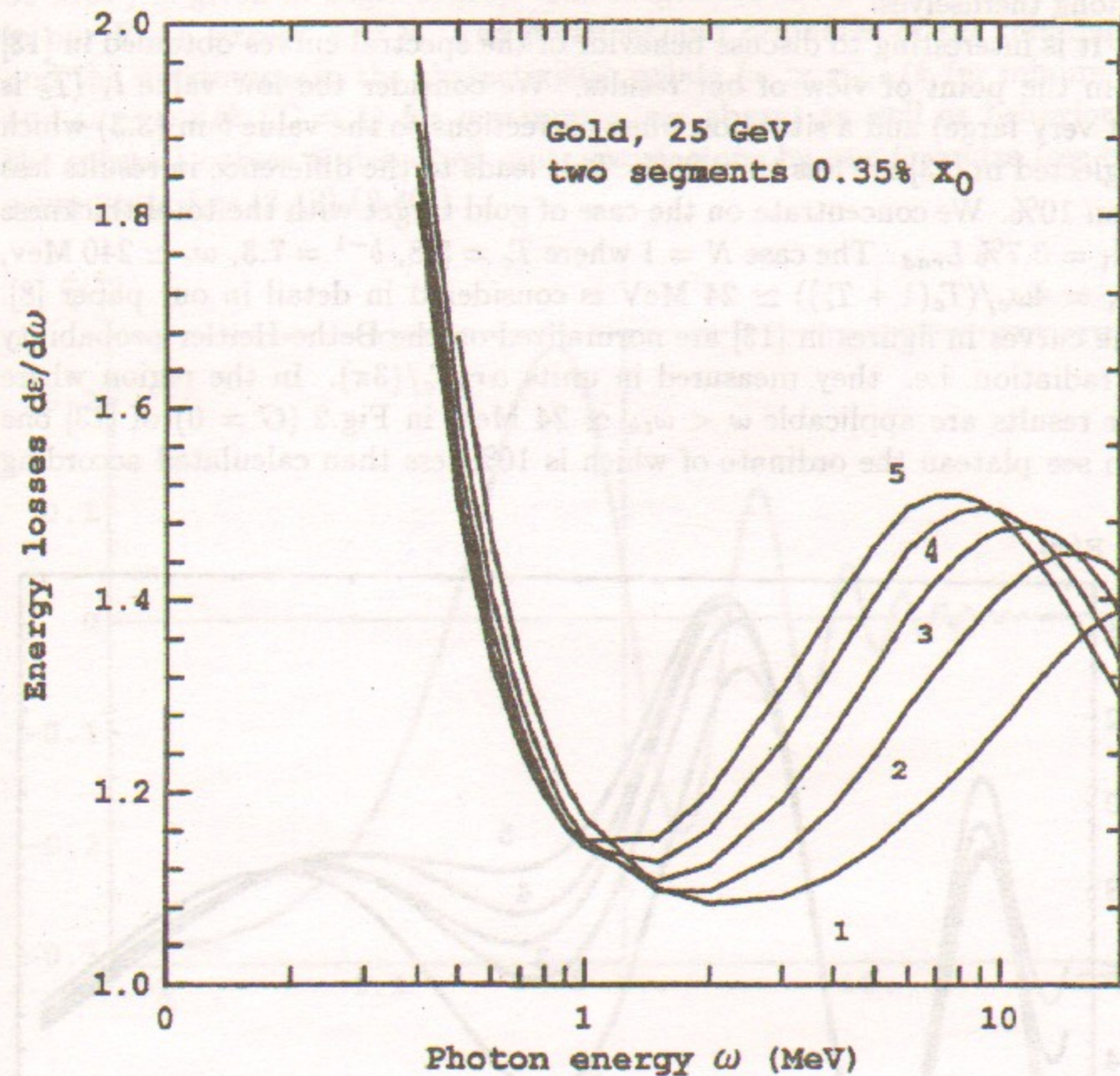
Figure 1: The energy losses spectrum \frac{d\epsilon}{d\omega} in units \frac{2\alpha}{\pi} , in the target consisting of two gold plates with thickness l_1 = 11.5 \mu\text{m} for the initial electrons energy \epsilon = 25 GeV:
