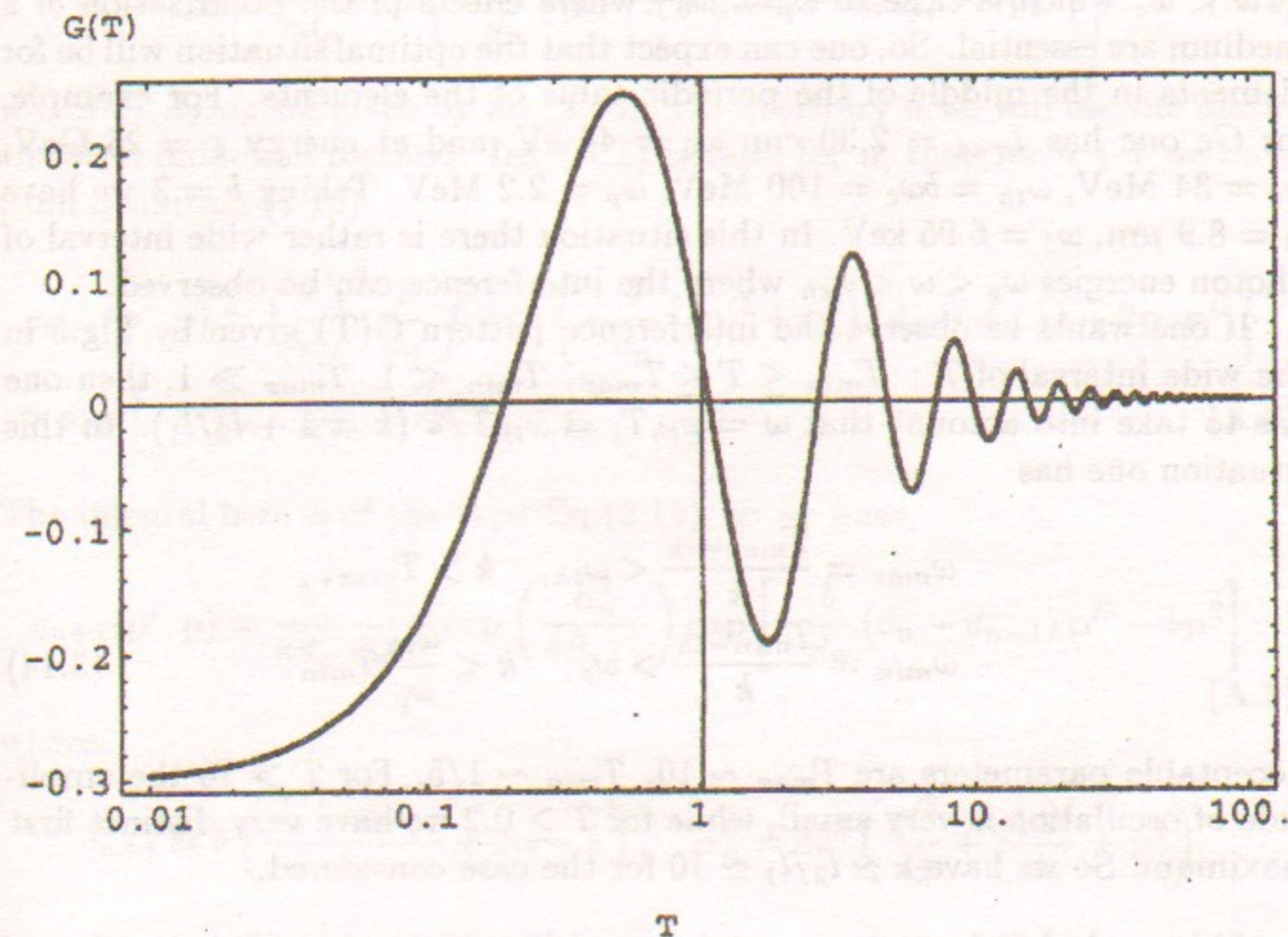
Figure 3: The function G(T) (2.37).
