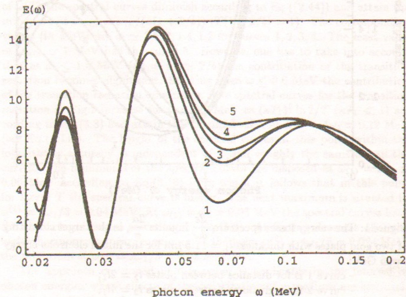
Figure 2: The same as in Fig.1 E(\omega) = \frac{d\varepsilon}{d\omega} in soft part of the spectrum where transition radiation contributes only.
