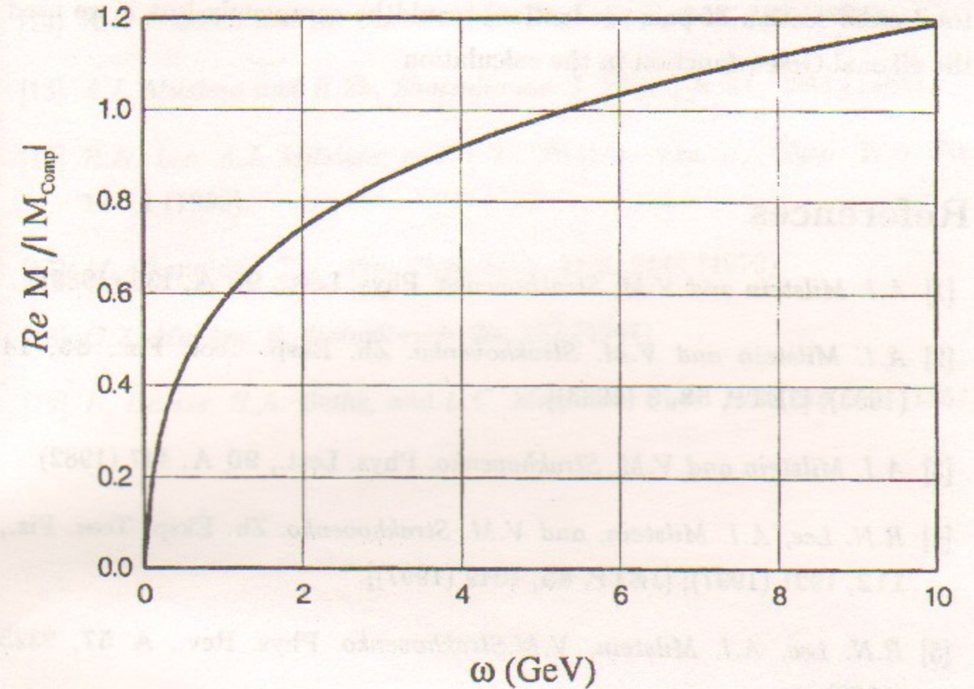
Figure 1: The real part of the forward Delbruck scattering amplitude for the potential V(r) = -Z\alpha \exp(-m\alpha Z^{1/3}r)/r in units of 4\pi Z\alpha/m , Z = 82 as a function of \omega .
