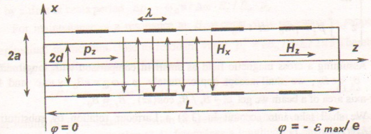
Fig. 3.1. A scheme of resonant recuperator.
