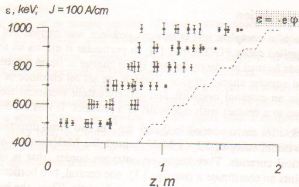
Fig. 3.2. Distribution of absorbed electrons on recuperator length; B_0 = 2.5 kGs, \varepsilon_0 \sim 180 keV, \varepsilon_z^0 = 100 keV, \eta = 62\% .
