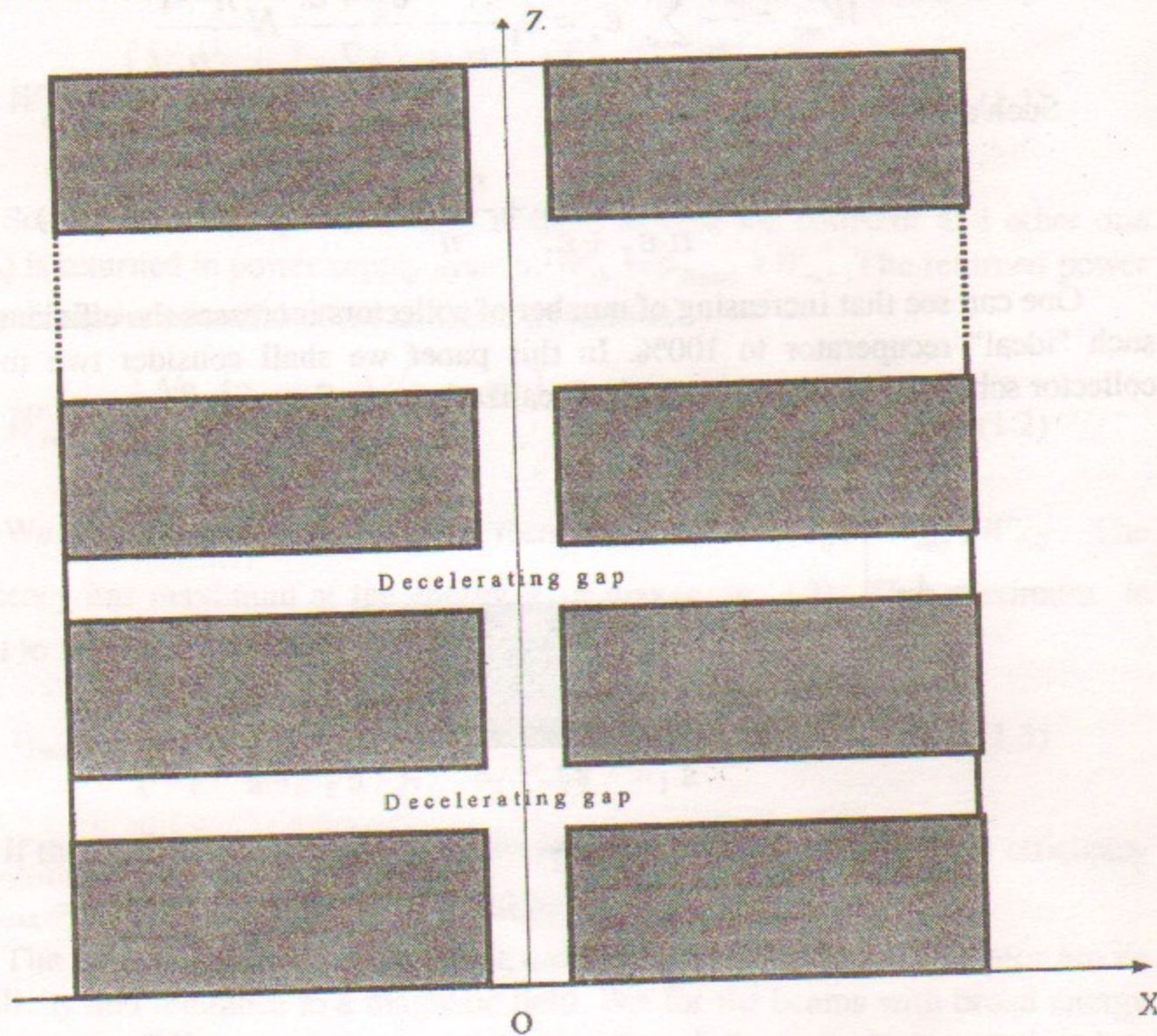
Fig. 2.1. The basic scheme of sectioned recuperator.
