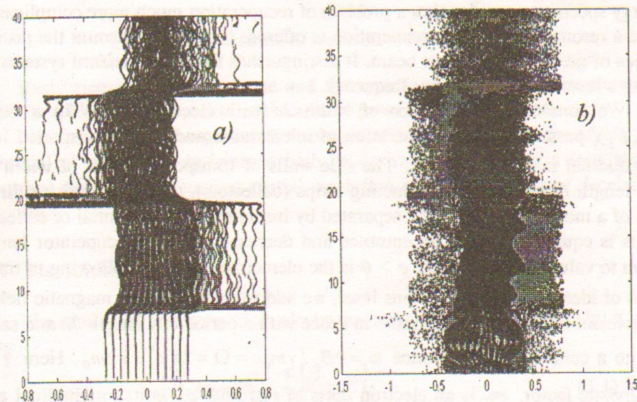
Fig. 2.6 a) and b). Nonself-consistent and self-consistent motion of an electron beam through recuperator for separating fields values B_x=1.15 kGs, B_z=0.8 kGs.
