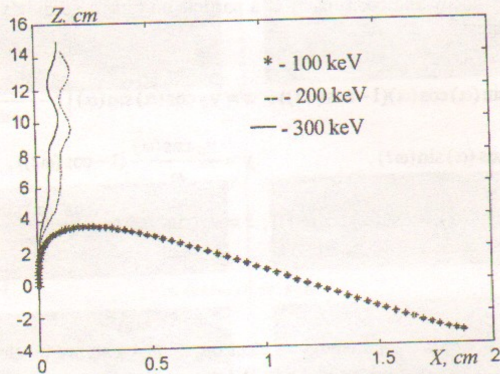
Рис.2.2. Trajectory of particles with different energy in a constant magnetic field, dependent on coordinate z :
