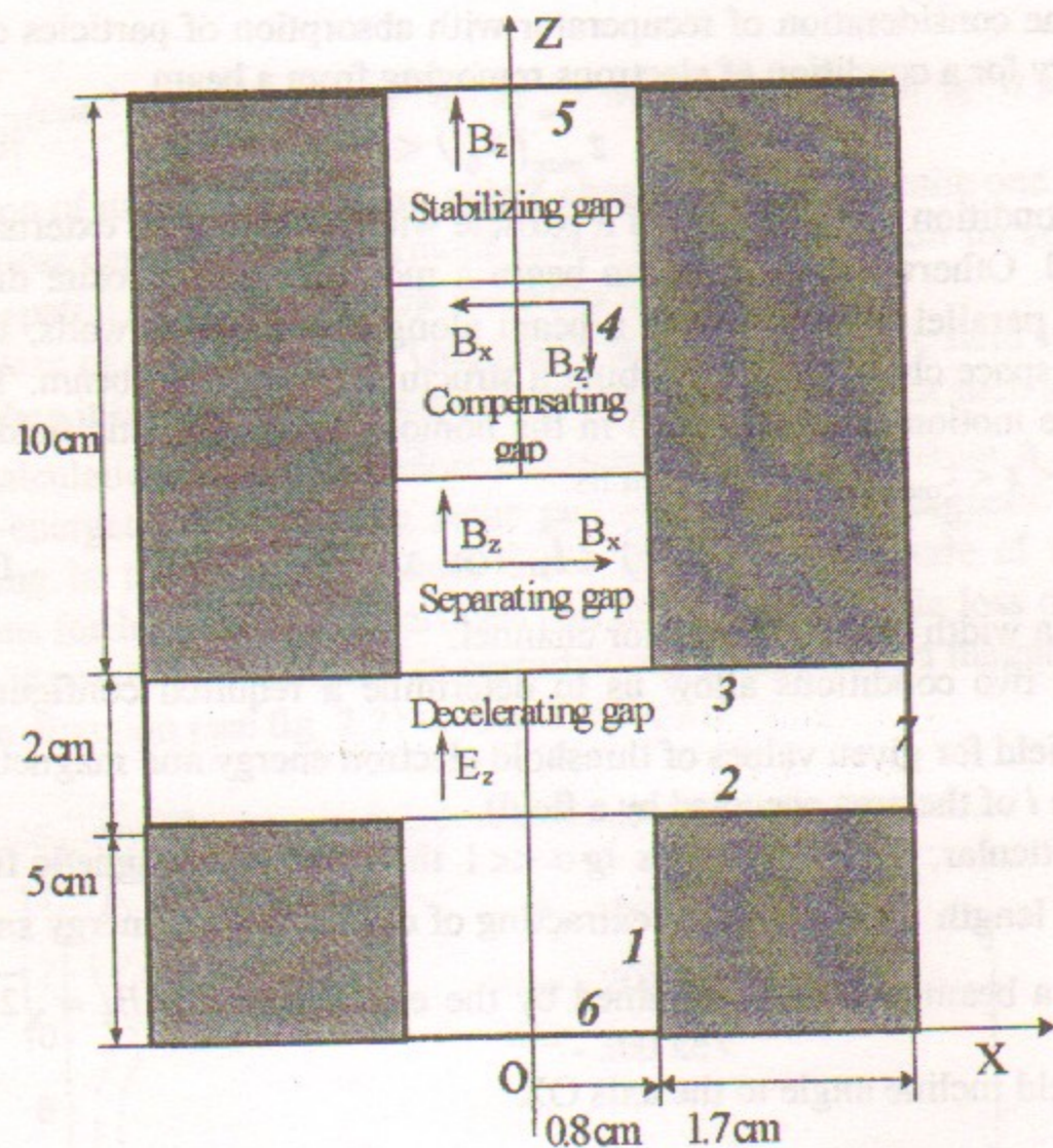
Fig. 2.3. The basic scheme of a recuperator section.
