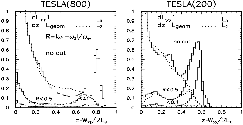
Figure 2: \gamma\gamma luminosity spectra at TESLA. Solid line for total helicity of the two photons 0 and dotted line for total helicity 2. Dashed curves: luminosities with cuts on longitudinal momentum. See the text.
