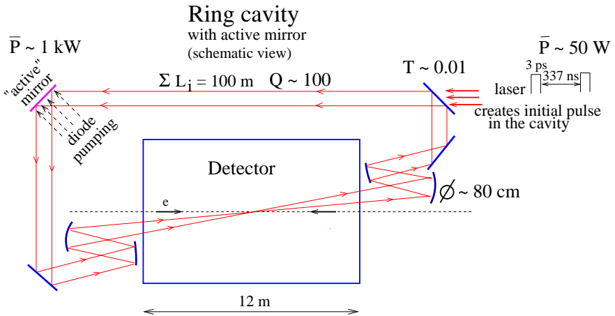
Figure 5: Ring type “external” optical cavity for the photon collider at TESLA (only optics for conversion of one electron beam is shown).
