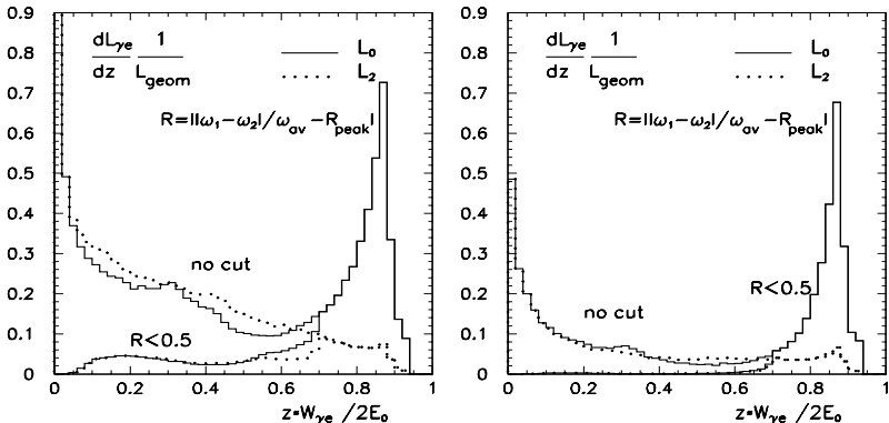
Figure 3: Normalized \gamma e luminosity spectra at TESLA(500). Left: the photon collider is optimized for \gamma\gamma collisions; right: one electron beam is converted and the distance between IP and CP is 1.05 cm, 5 times larger than for the left figure.
