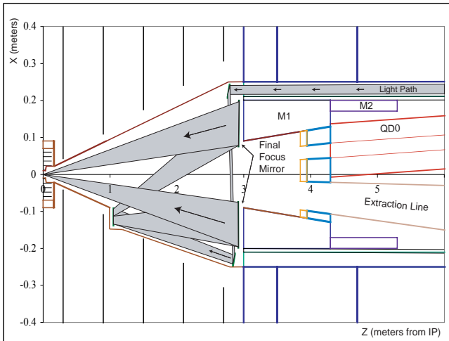
Figure 6: Laser optics at the NLC interaction region.
