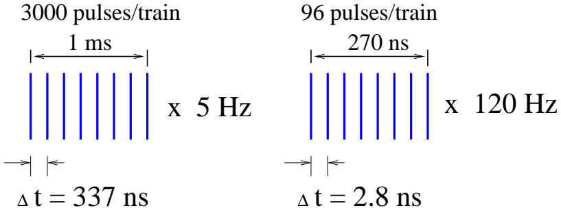
Figure 4: Structure of electron beams at TESLA(left) and NLC/JLC(right).
