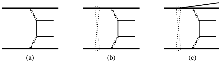
Figure 2: Modification of the elastic two-photon process by rescattering (final state rescattering is not shown).
