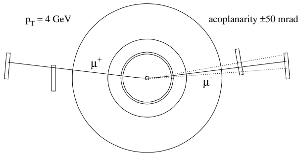
Figure 5: The common \mu^+\mu^- track in (\rho, \varphi) -projection (the multiple scattering is not taken into account).
