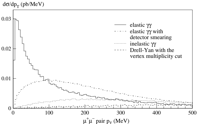
Figure 3: The differential dimuon cross section d\sigma/dp_T for pp \rightarrow pp + \mu^+\mu^- as a function of the pair transverse momentum p_T (ATLAS, W > 12 GeV, |\eta| < 2.3 ).
