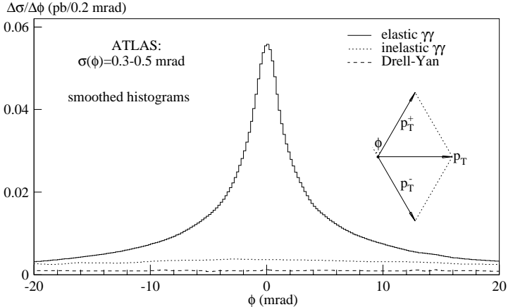
Figure 4: The acoplanarity distributions for the signal and dominant background processes with all cuts applied.
