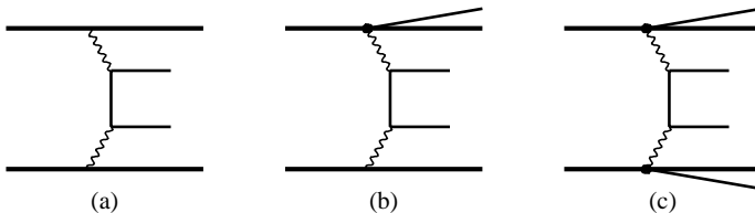
Figure 1: Two-photon production of lepton pairs in pp collisions: (a) - elastic, (b,c) - inelastic
