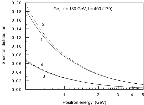
Fig. 1. The summary spectral distribution dw/dz = dw_2/dz + dw_c/dz of pair electroproduction in amorphous germanium at the initial electron energy \varepsilon = 180 GeV. In the curves 1 and 3 (for two target thicknesses l = 400 \mu\text{m} and l = 170 \mu\text{m} respectively) the multiple scattering is taken into account (Eq.(11)), while in the curves 2 and 4 the multiple scattering is neglected (Eq.(12)).
