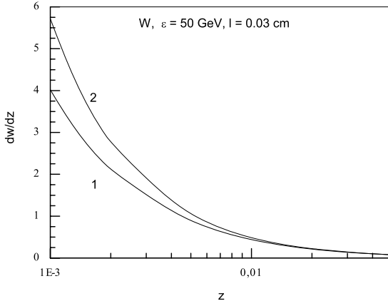
Fig. 4. The summary spectral distribution dw/dz = dw_2/dz + dw_c/dz of the pair electroproduction in amorphous tungsten of the thickness l = 300 \mu\text{m} ( 8.6\% L_{rad} ) at the initial electron energy \varepsilon = 50 \text{ GeV} . In the curve 1 the multiple scattering is taken into account (Eq.(11)), while in curve 2 the multiple scattering is neglected (Eq.(12)).
