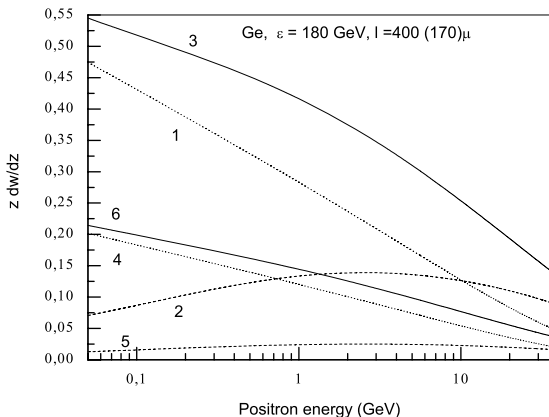
Fig. 2. The combination zdw/dz for the pair electroproduction probability in amorphous Ge at the initial electron energy \varepsilon = 180 GeV. The dotted curves 1 and 4 are the contributions of two-photon diagrams Eq.(3), the dashed curves 2 and 5 are the contributions of cascade process Eq.(11), the solid curves 3 and 6 are the sum of two previous contributions for two thicknesses l = 400 \mu\text{m} and l = 170 \mu\text{m} respectively. For convenience the ordinate is multiplied by 10^3 .
